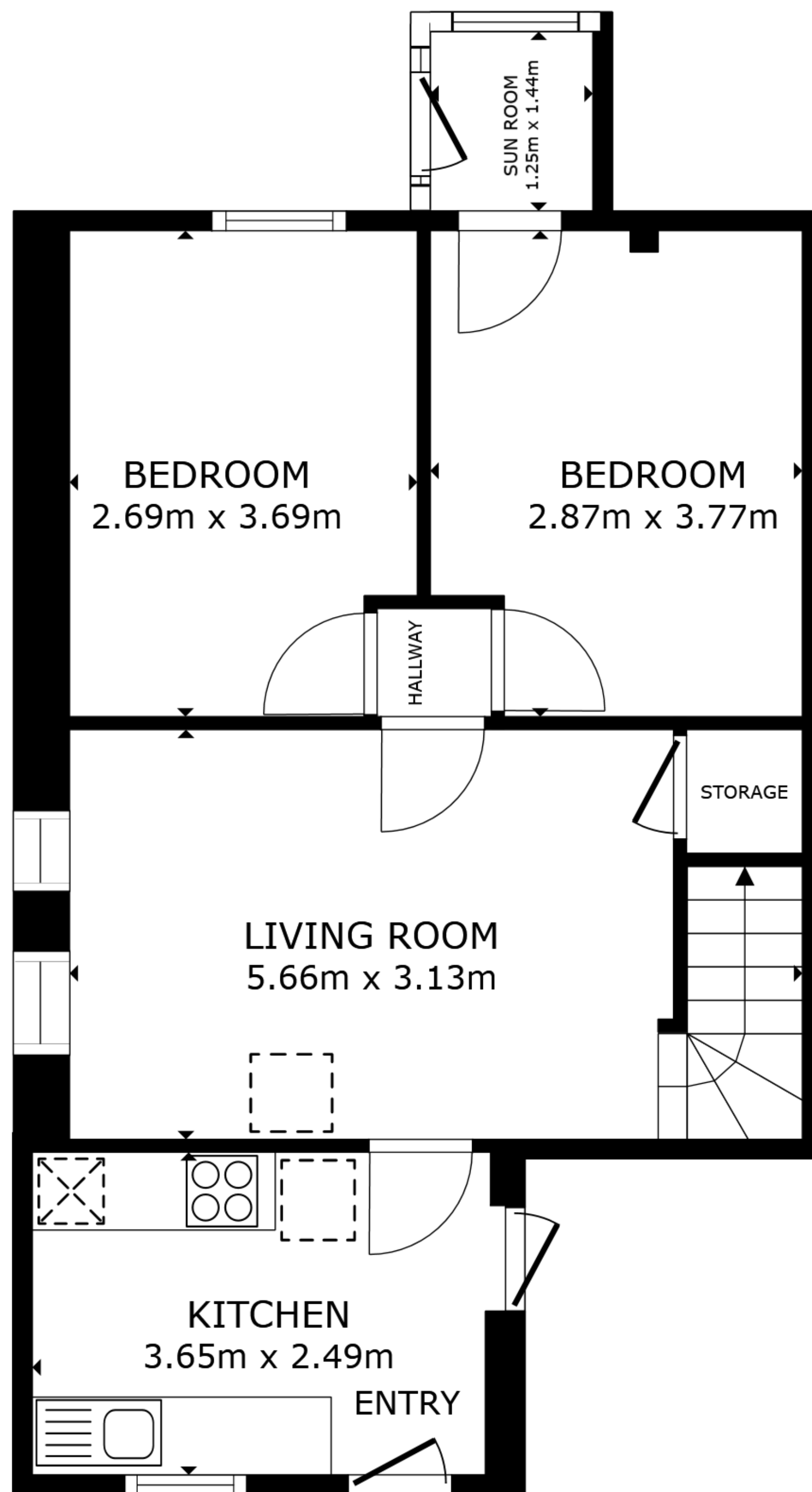
FLOOR 1
