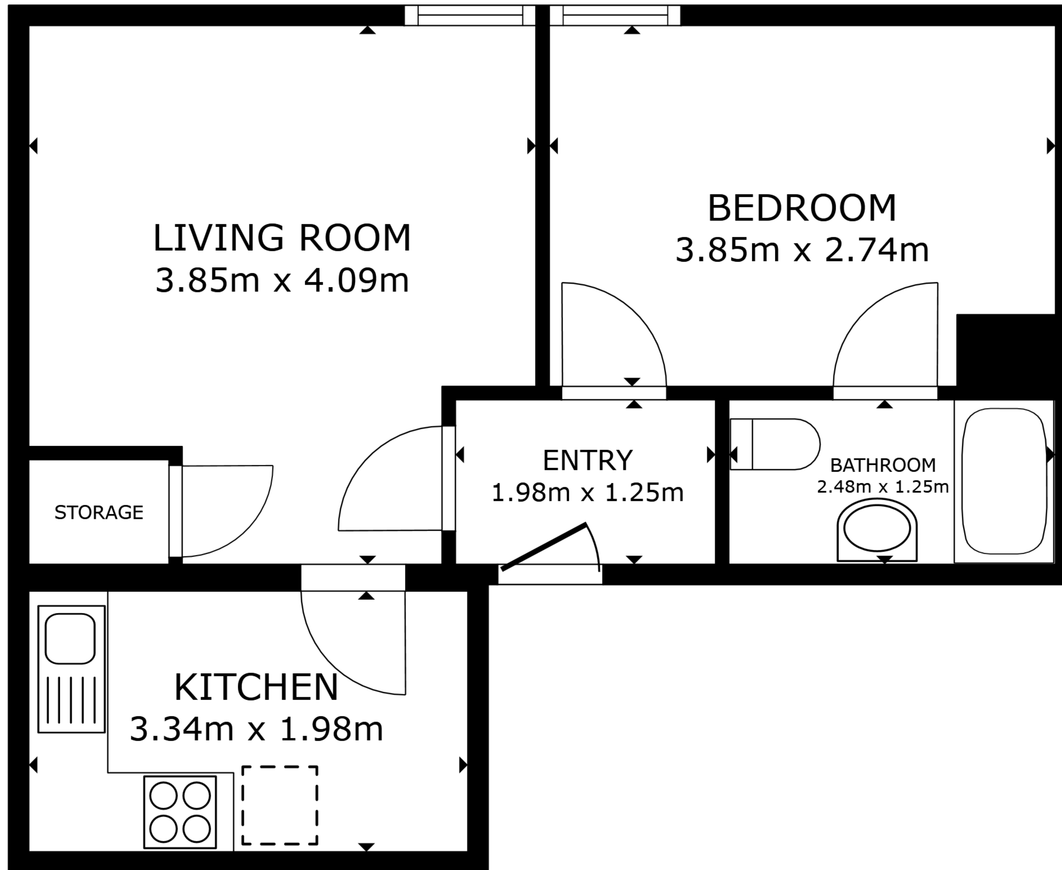
FLOOR PLAN
