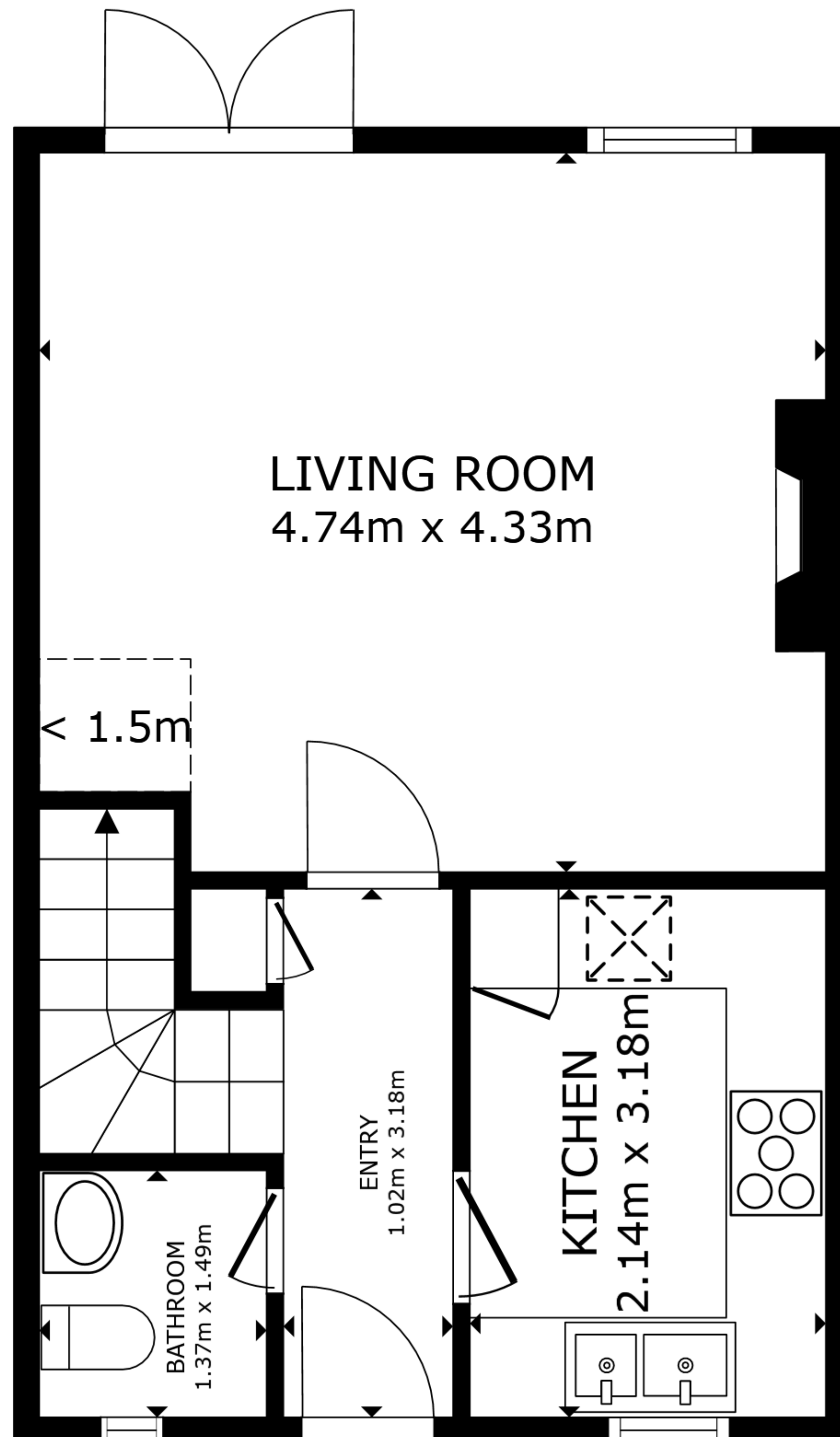
FLOOR 1
