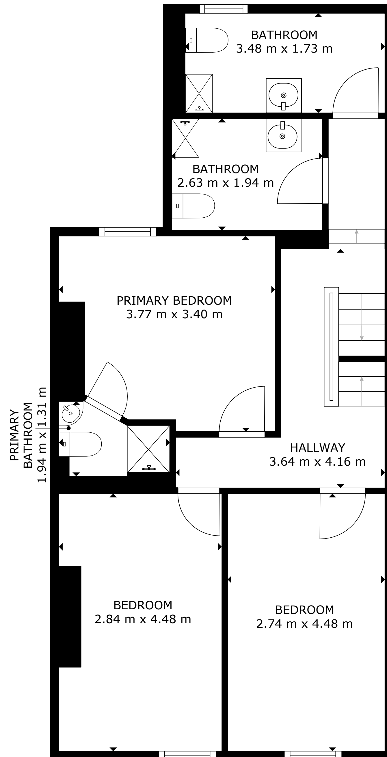
FLOOR 2
