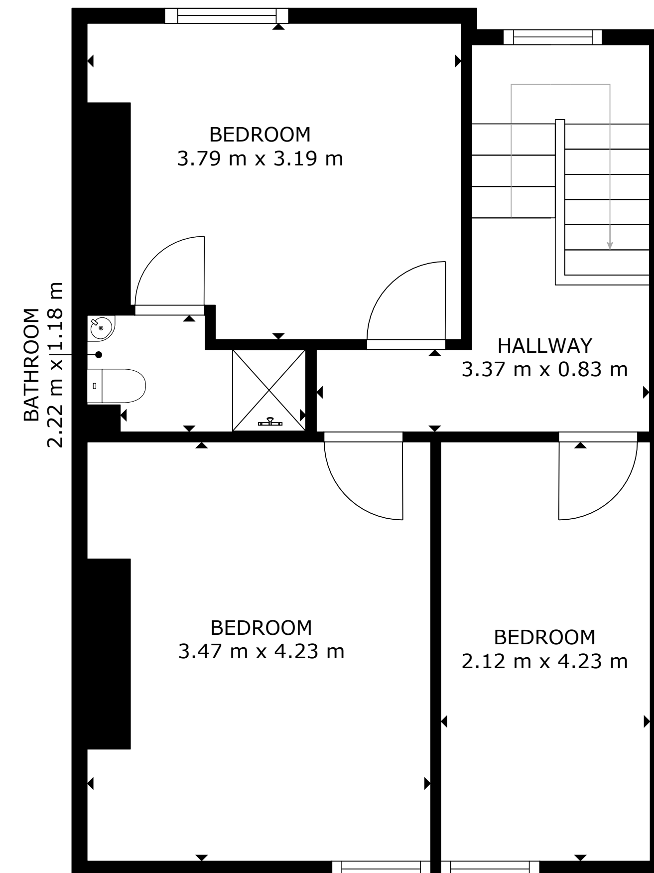
FLOOR 3
