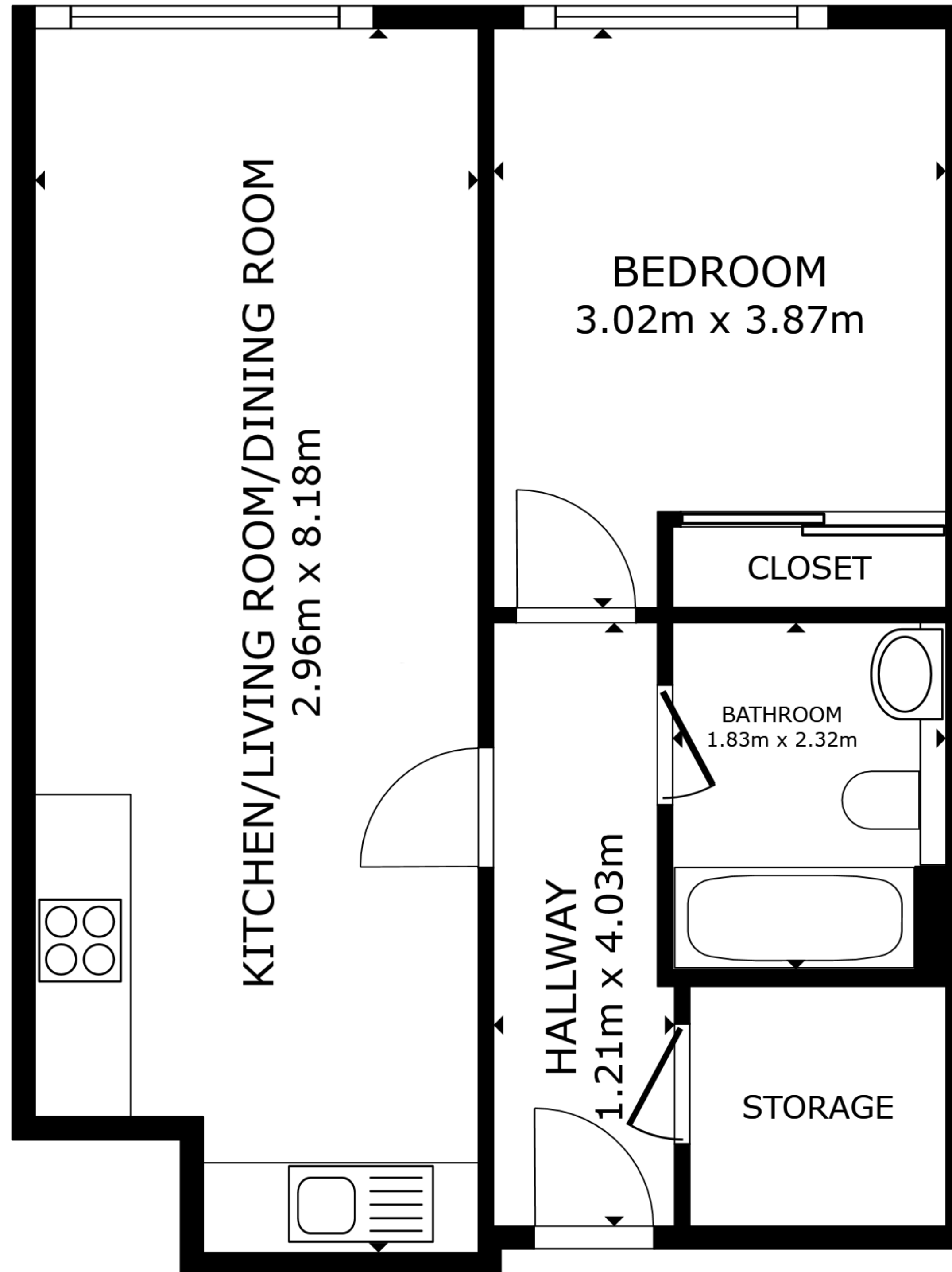
FLOOR PLAN
