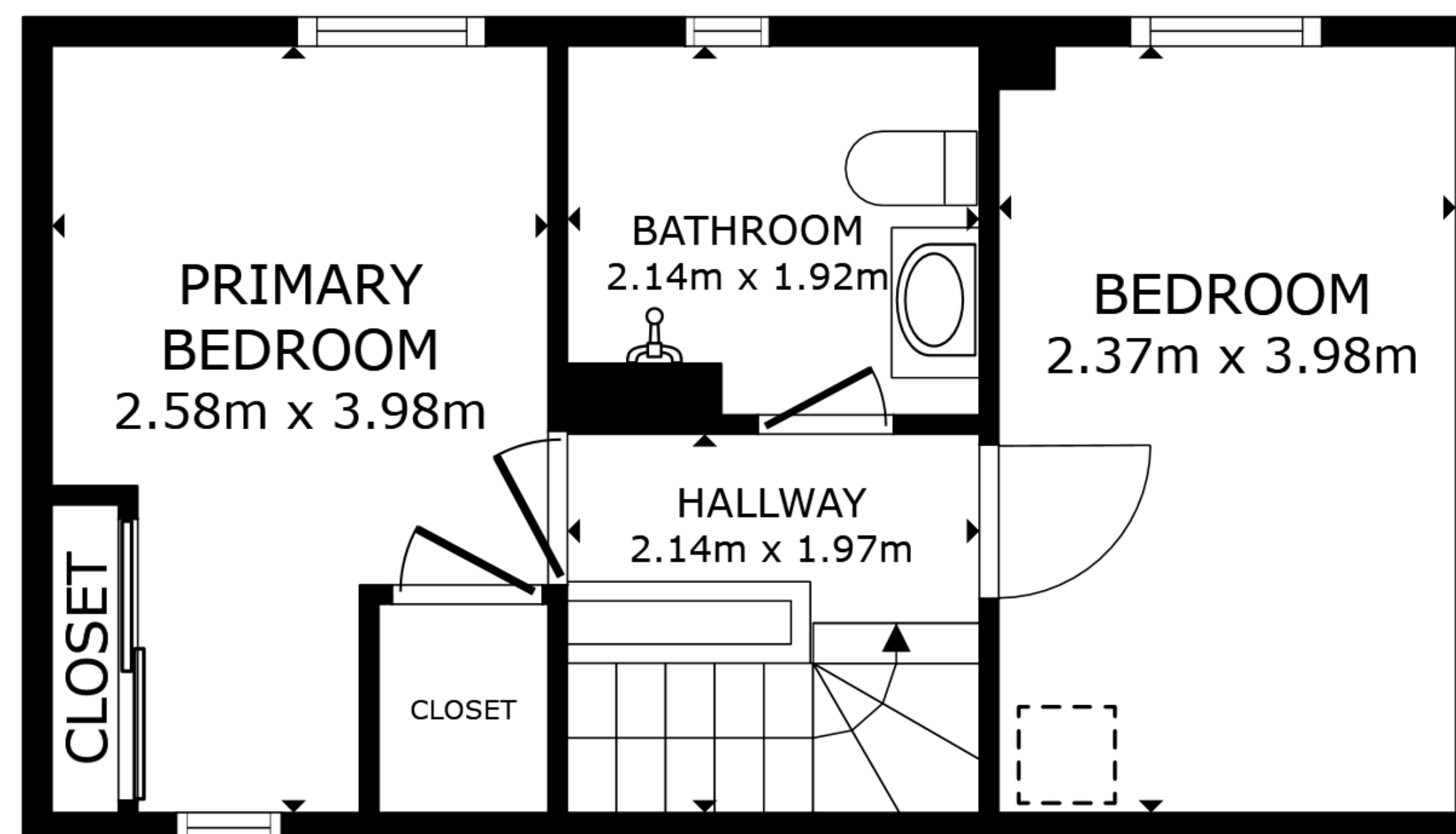
FLOOR 2
