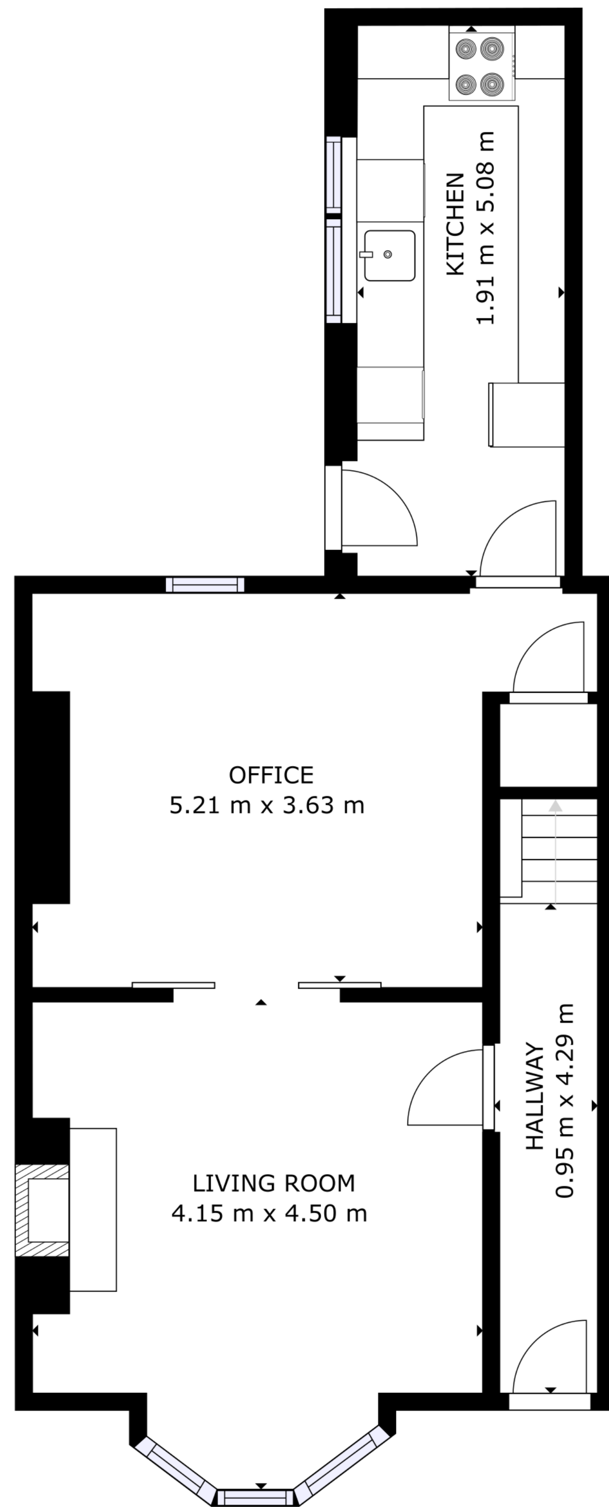
FLOOR 1
