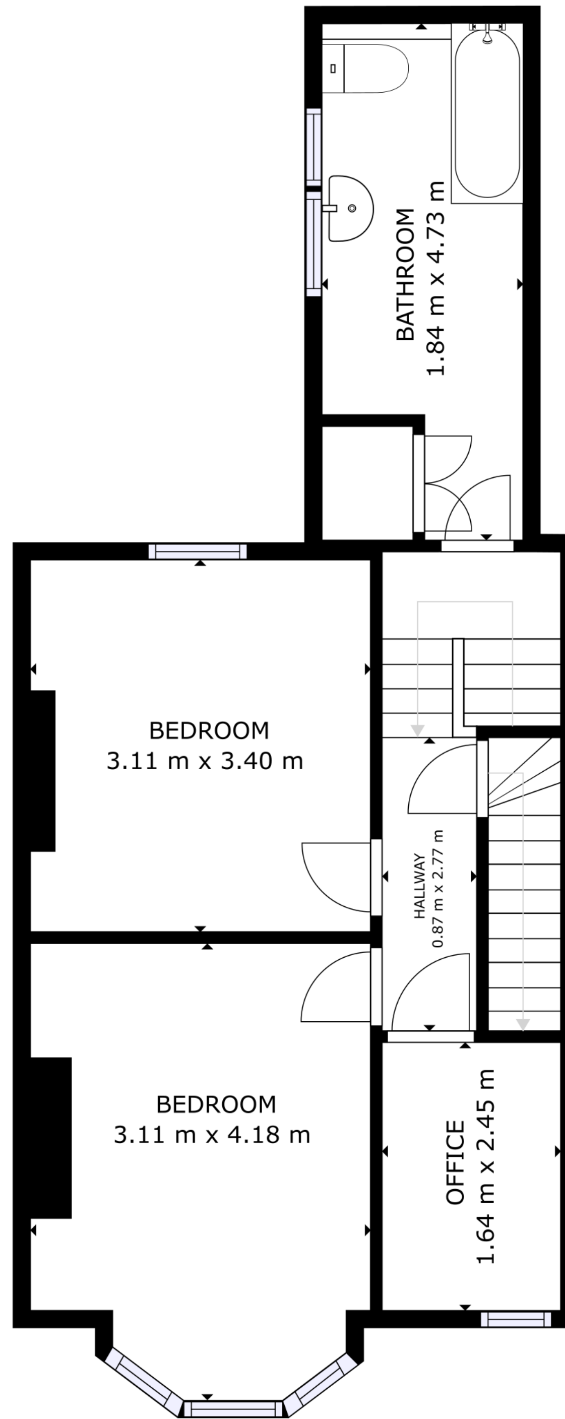
FLOOR 2
