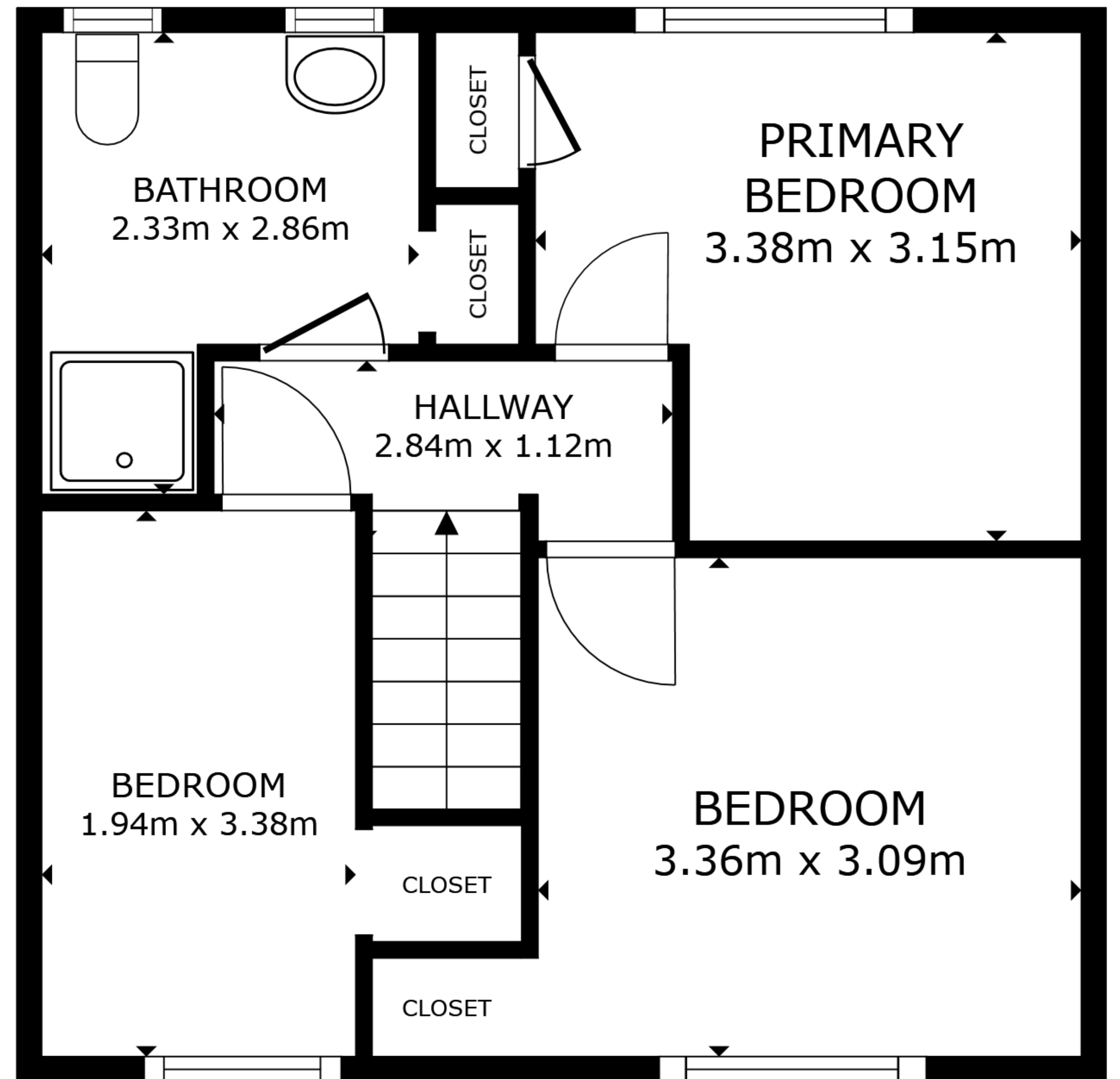
FLOOR 2
