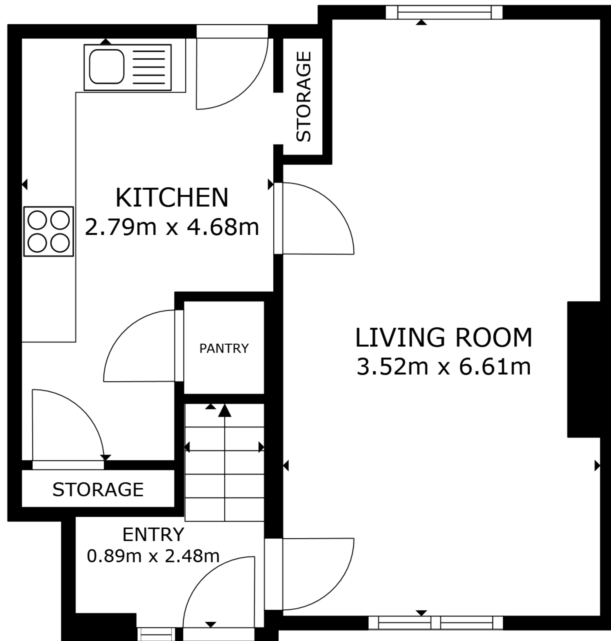
FLOOR 1
