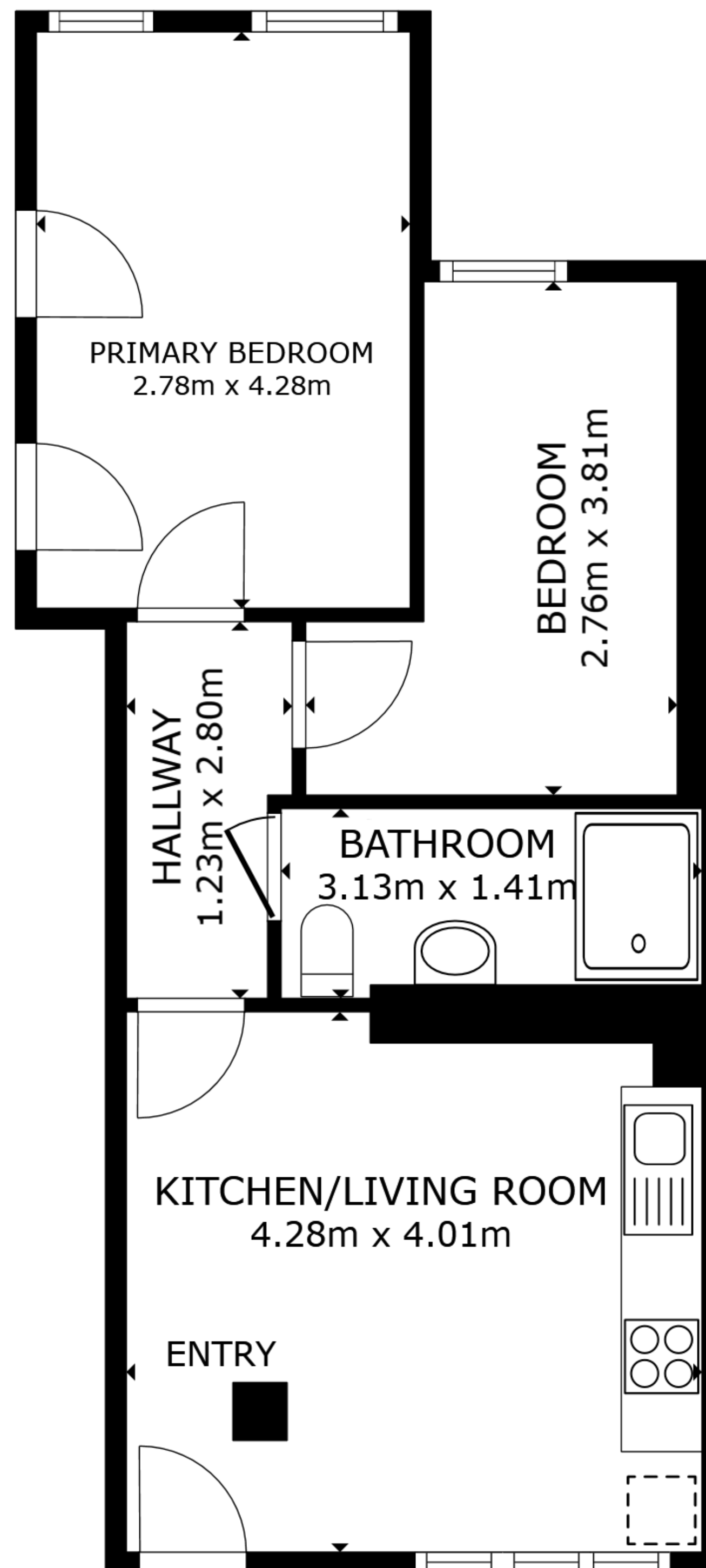
FLOOR PLAN
