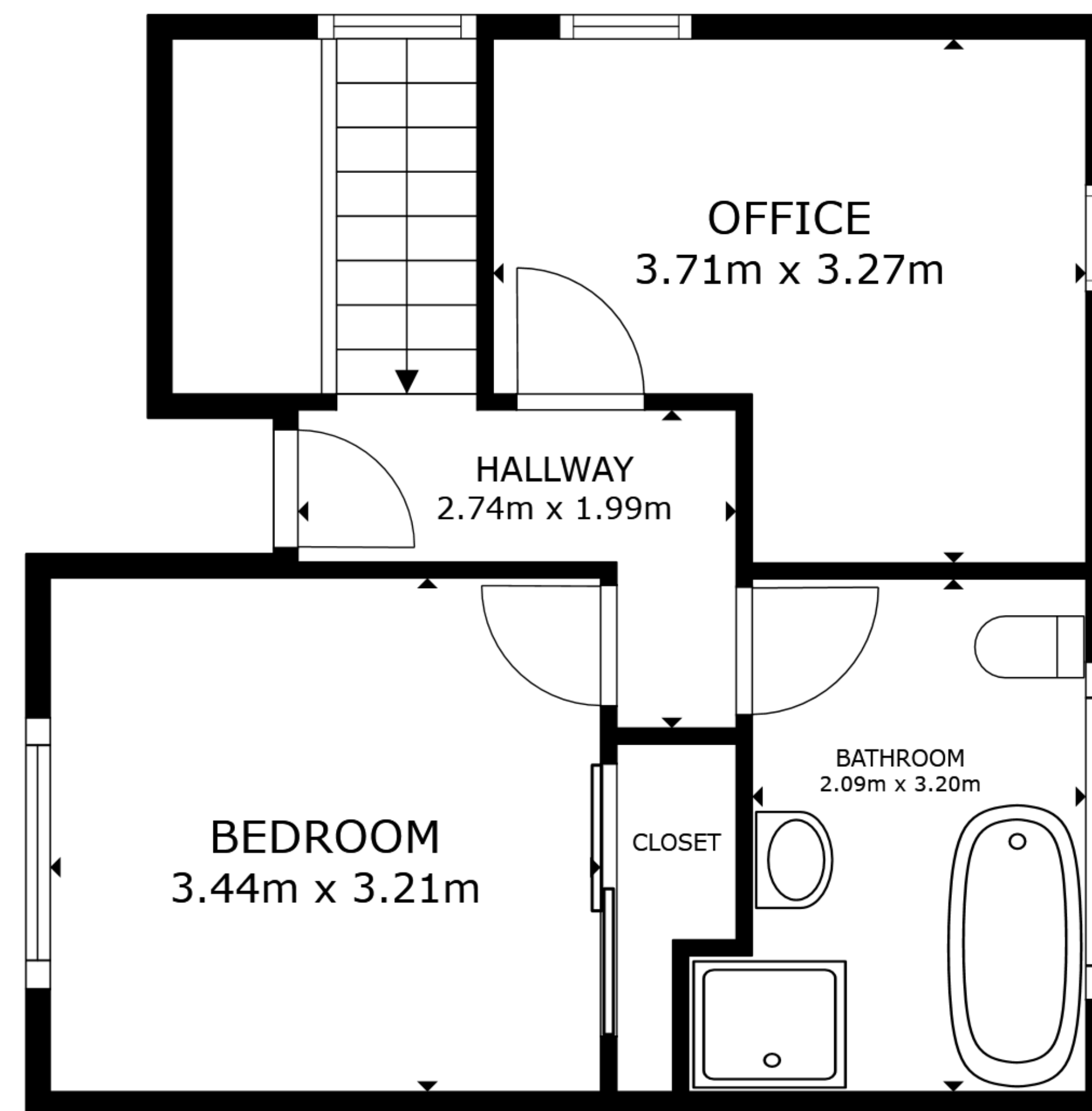
FLOOR 2
