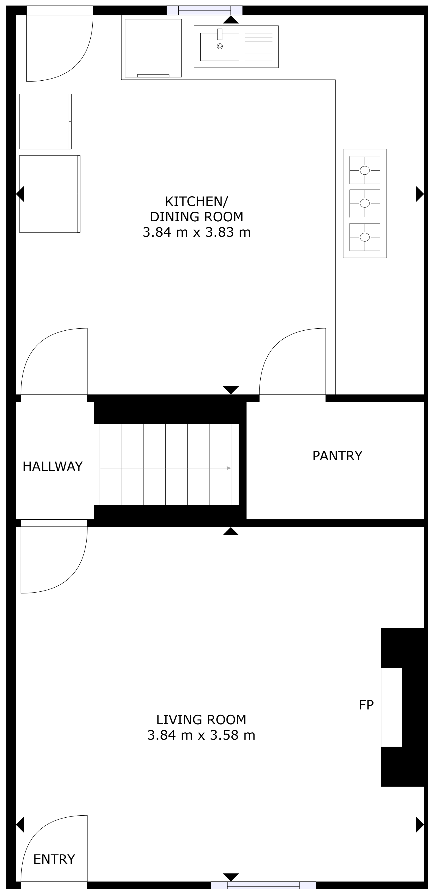
FLOOR 1
