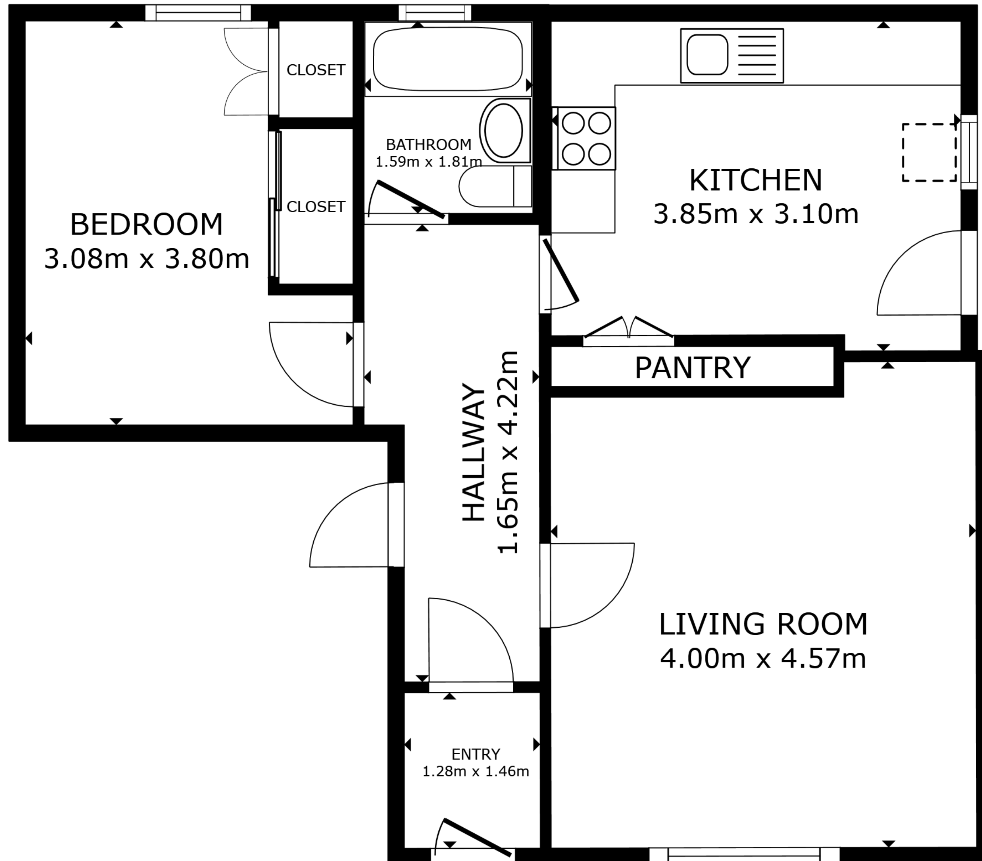
FLOOR PLAN
