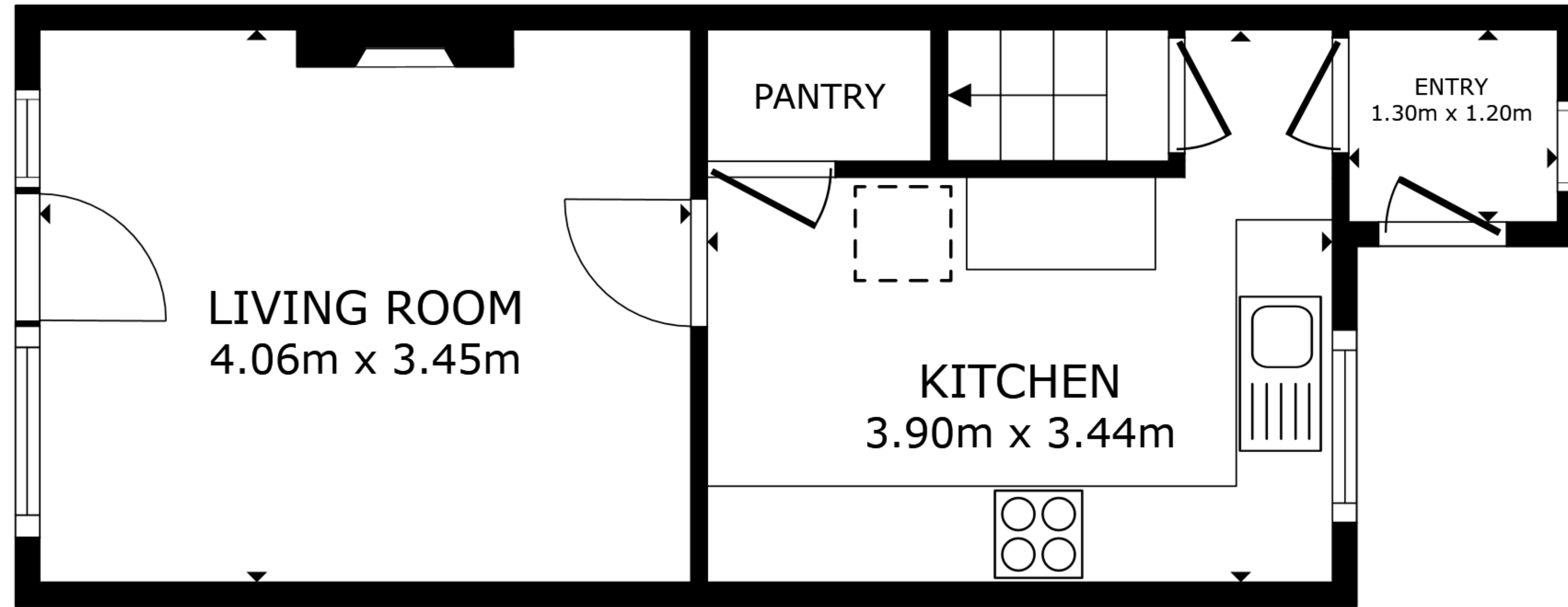
FLOOR 1
