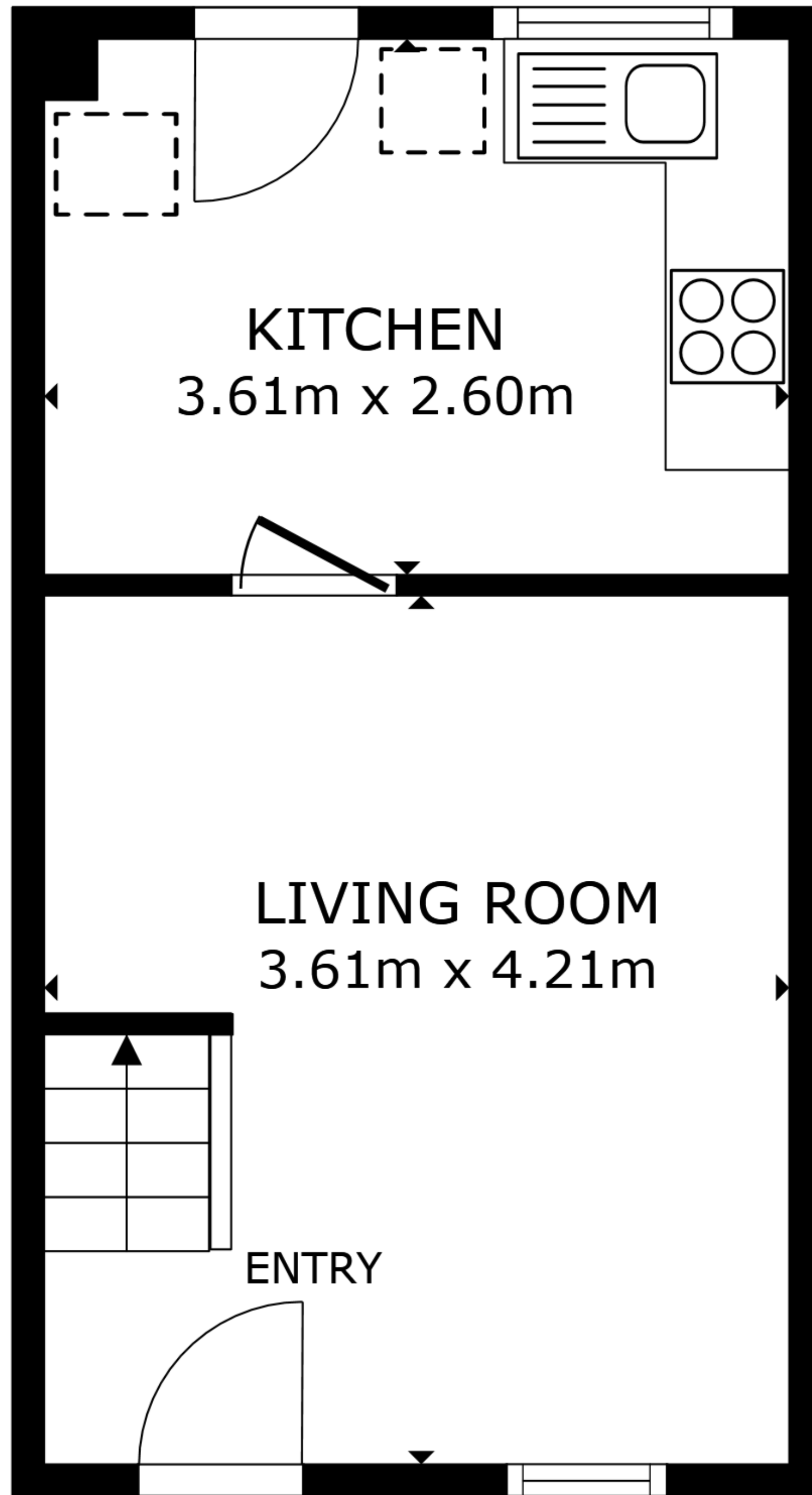
FLOOR 1
