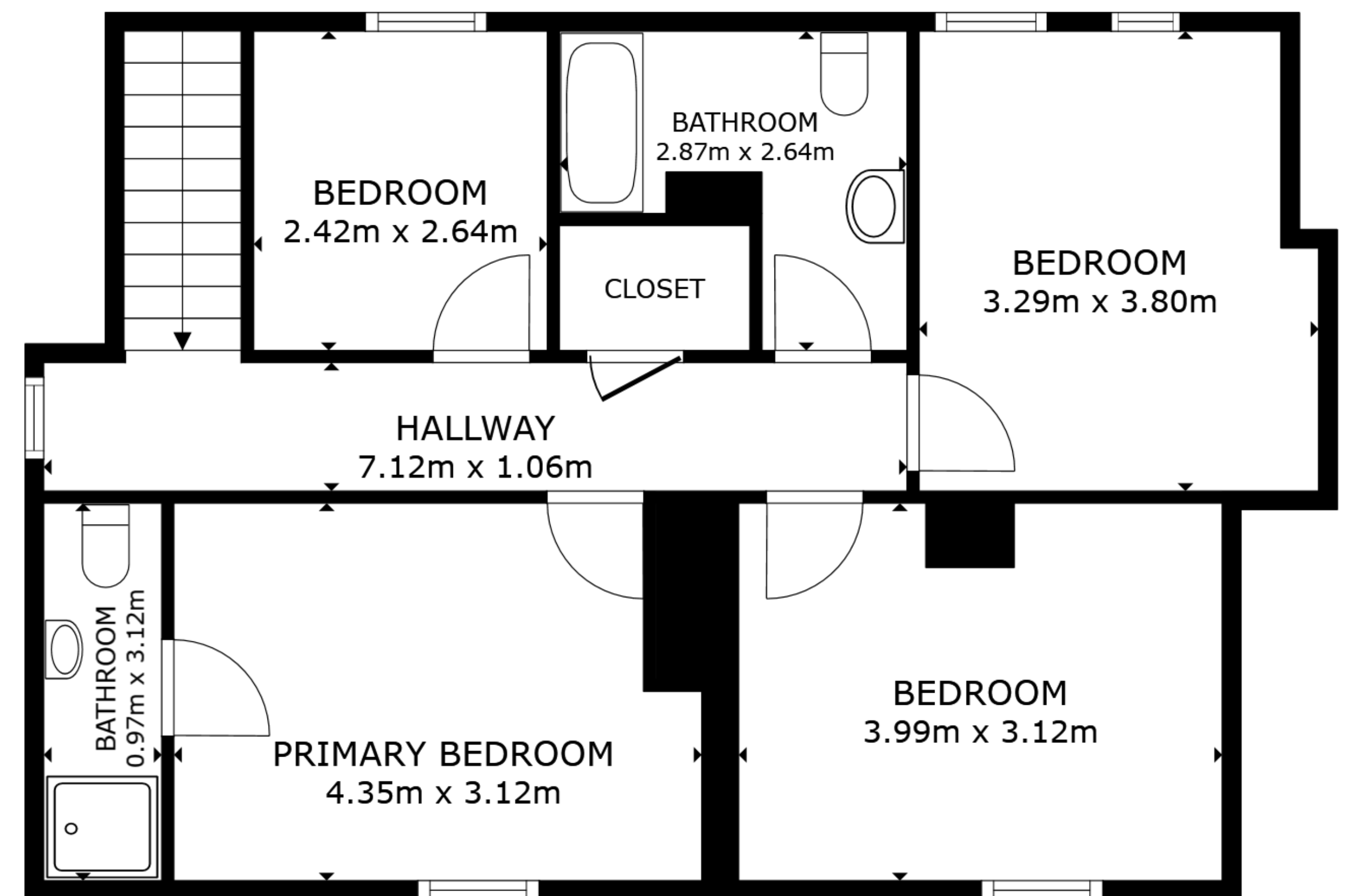
FLOOR 2
