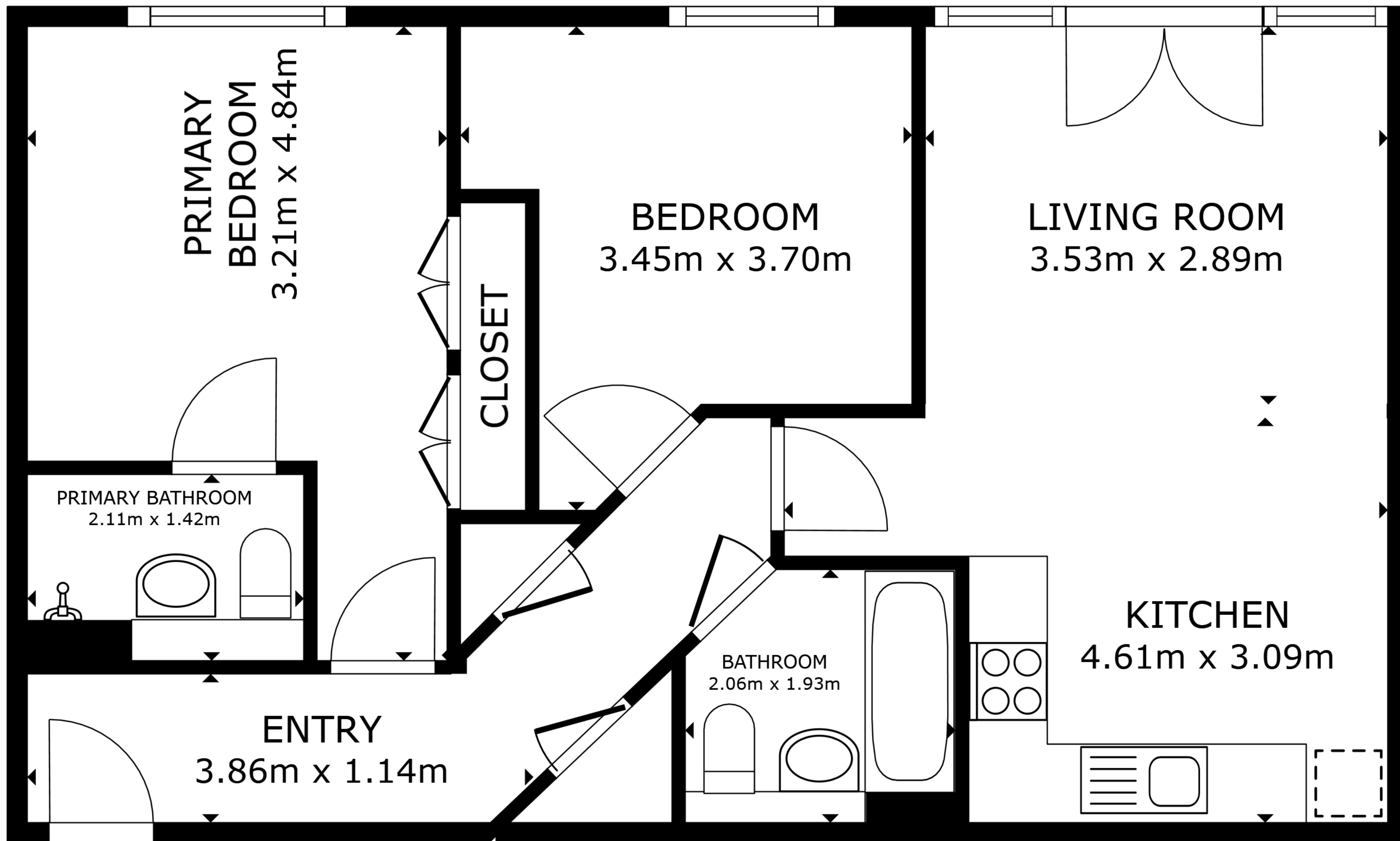
FLOOR PLAN
