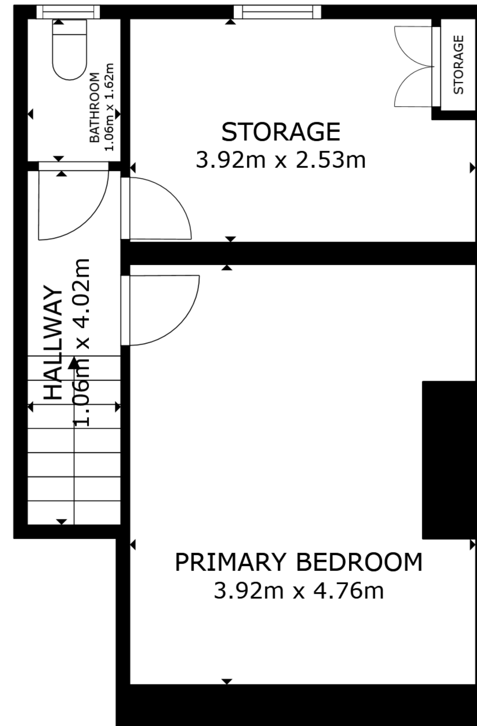
FLOOR 2
