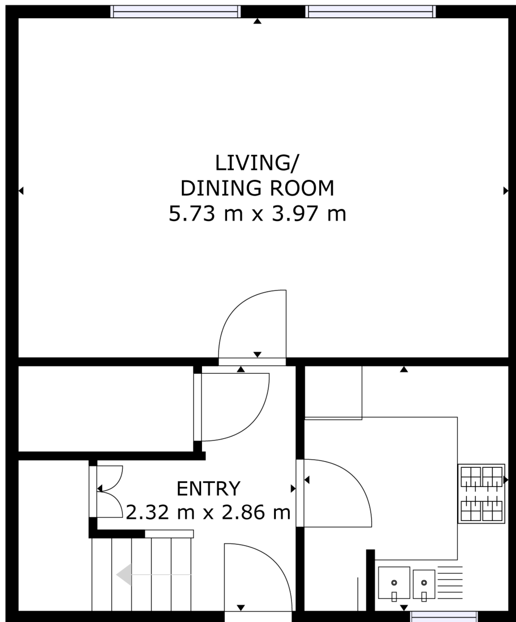
FLOOR 1
