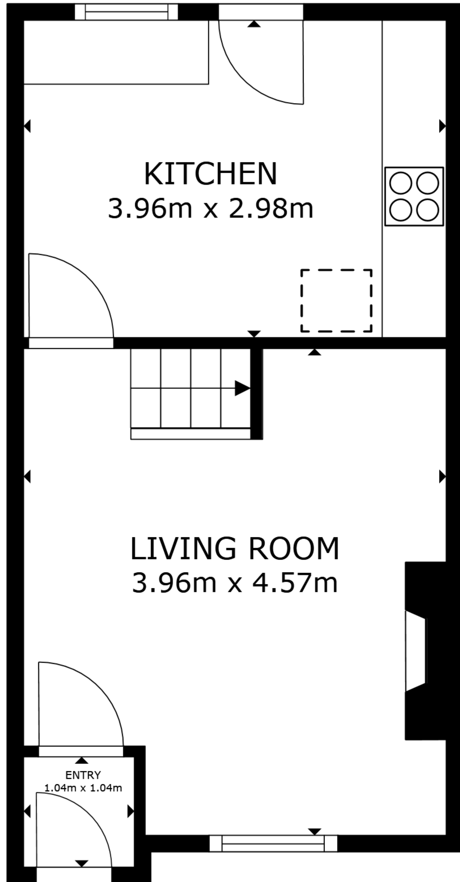
FLOOR 1
