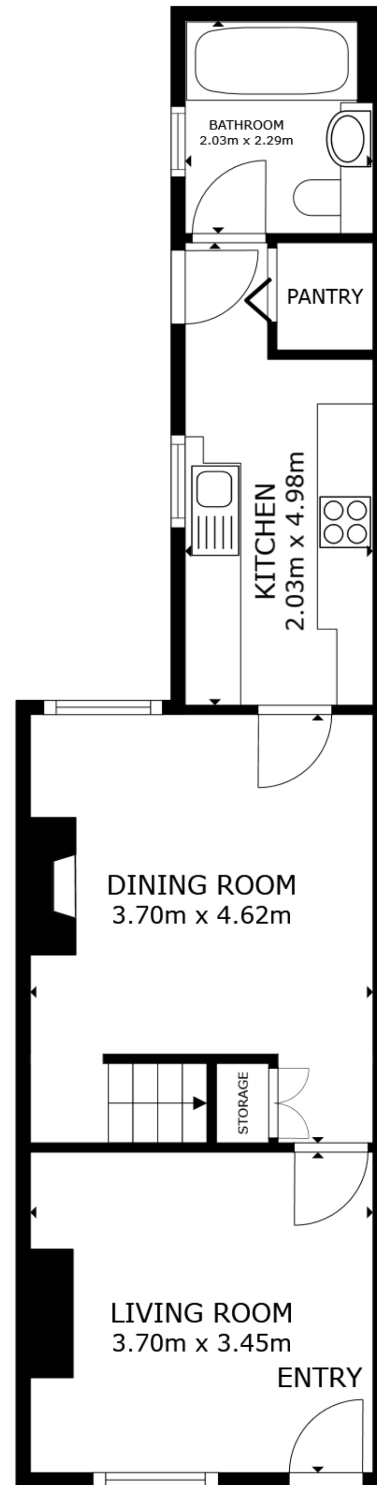
FLOOR 1
