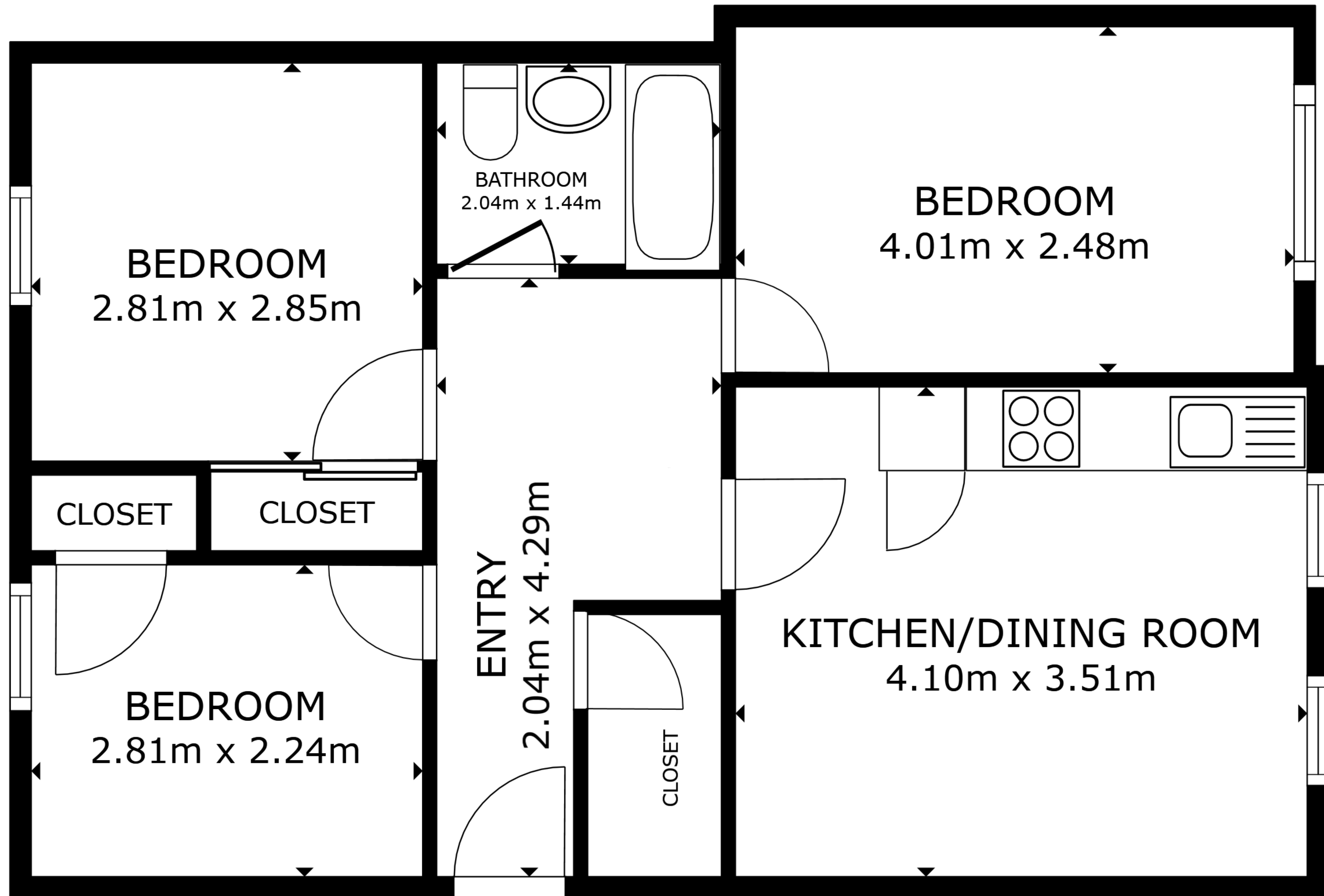
FLOOR PLAN
