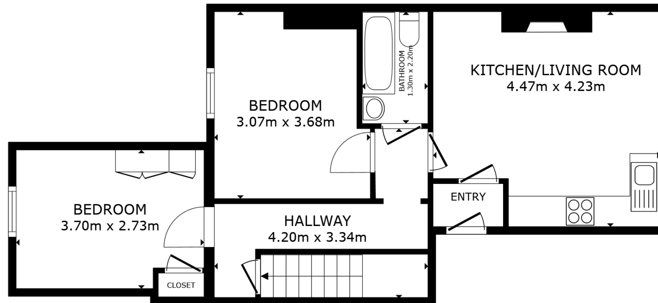
FLOOR 2
