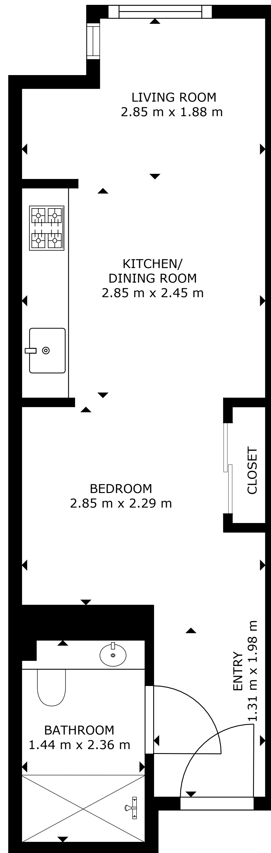
FLOOR PLAN
