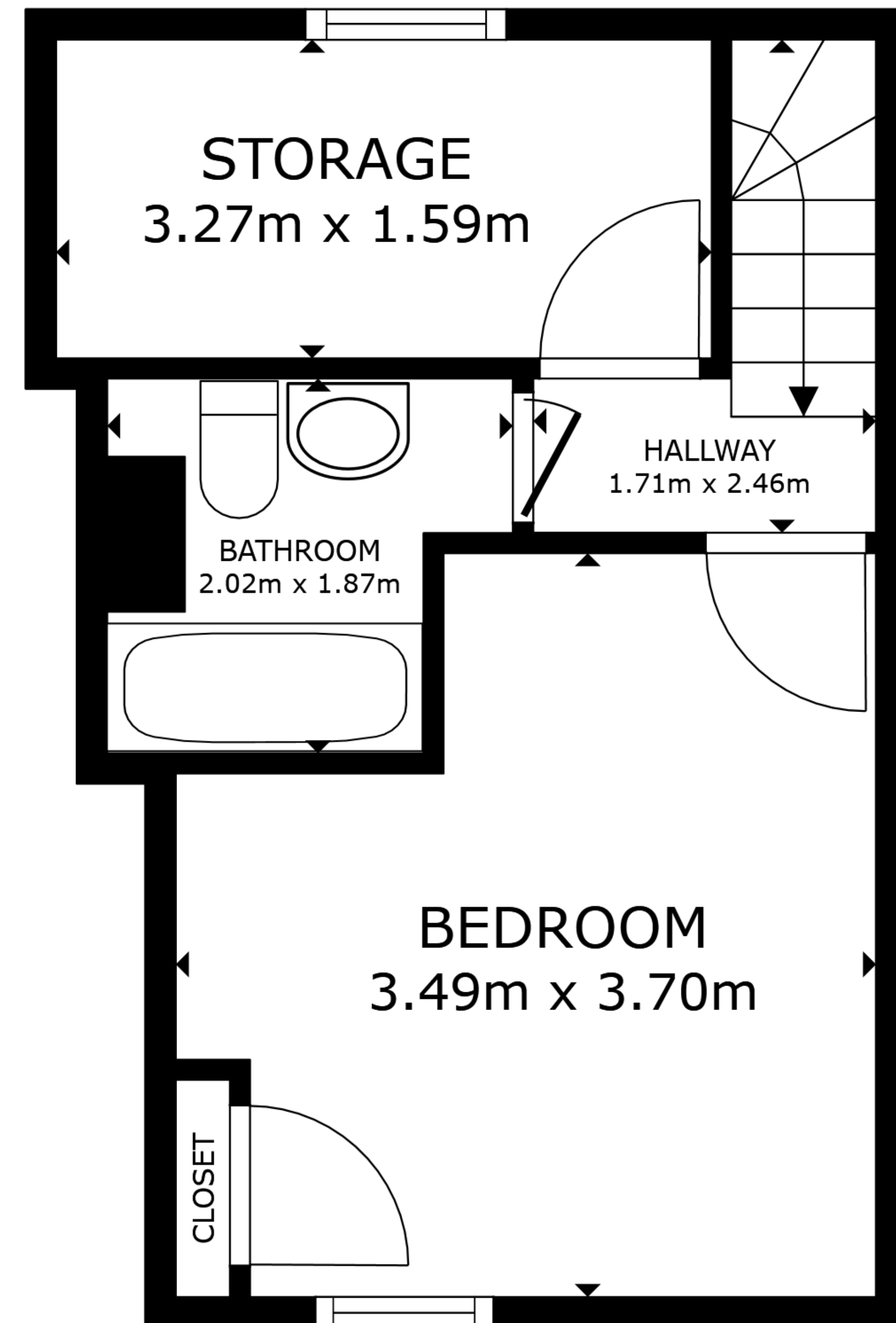
FLOOR 2
