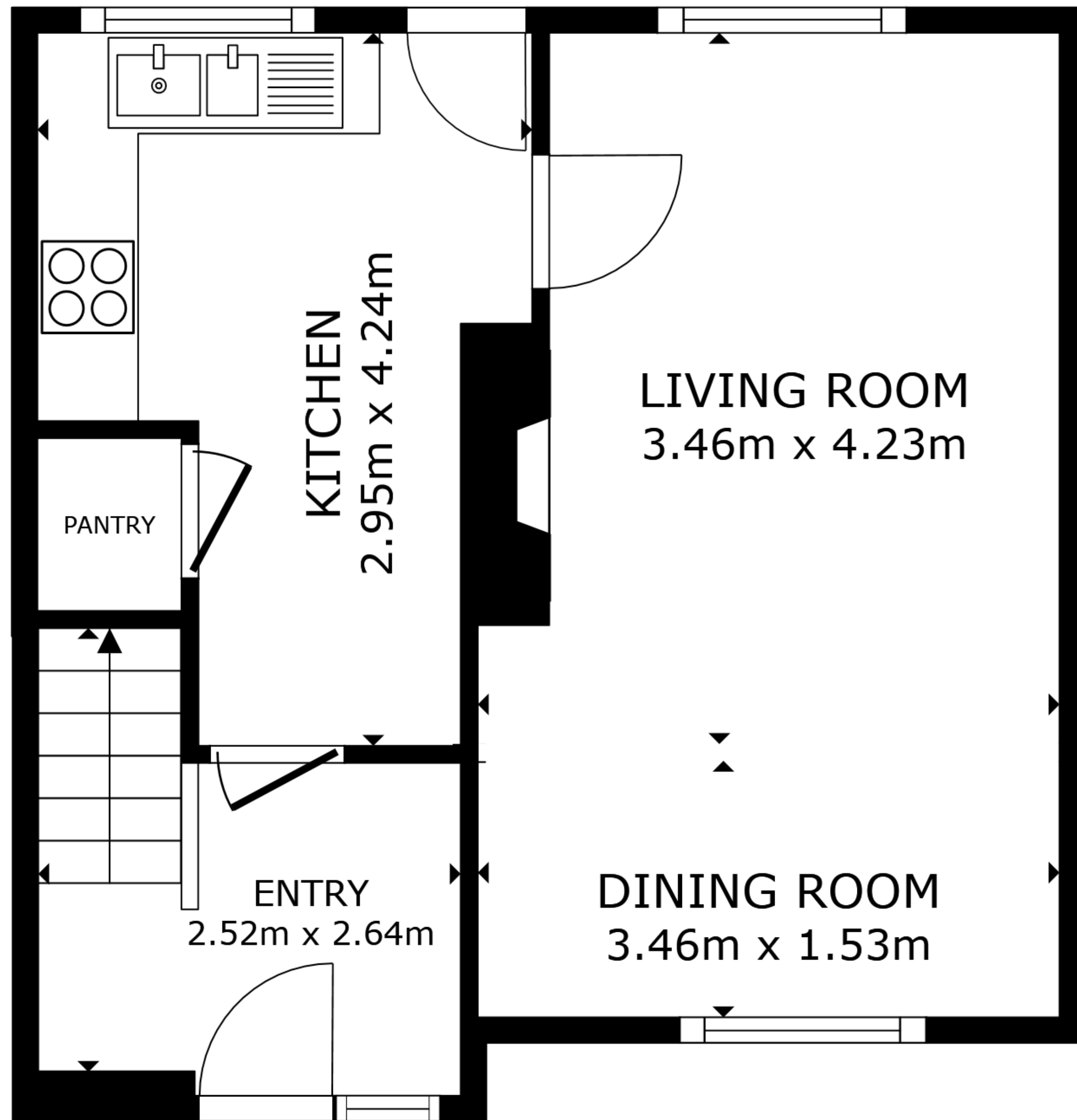
FLOOR 1
