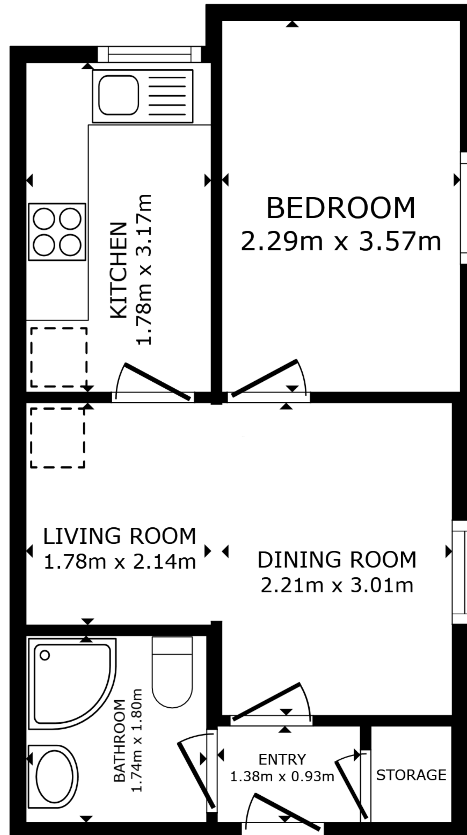
FLOOR PLAN
