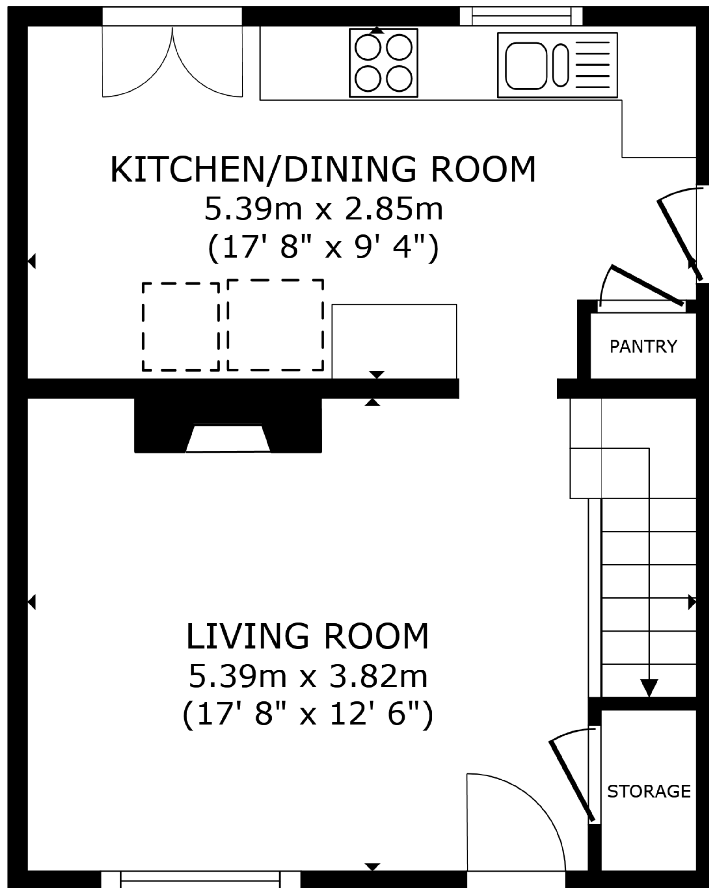
FLOOR 1
