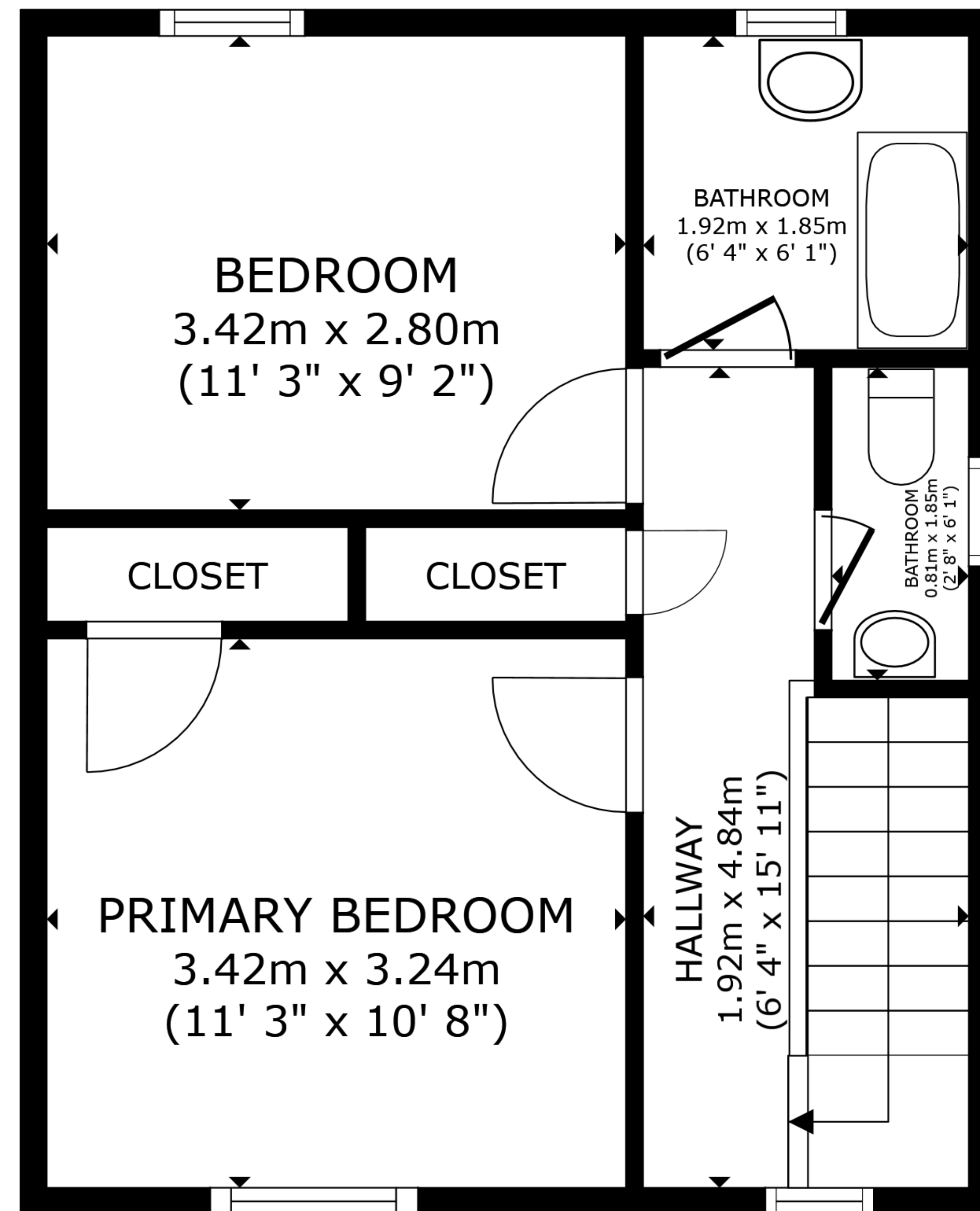
FLOOR 2
