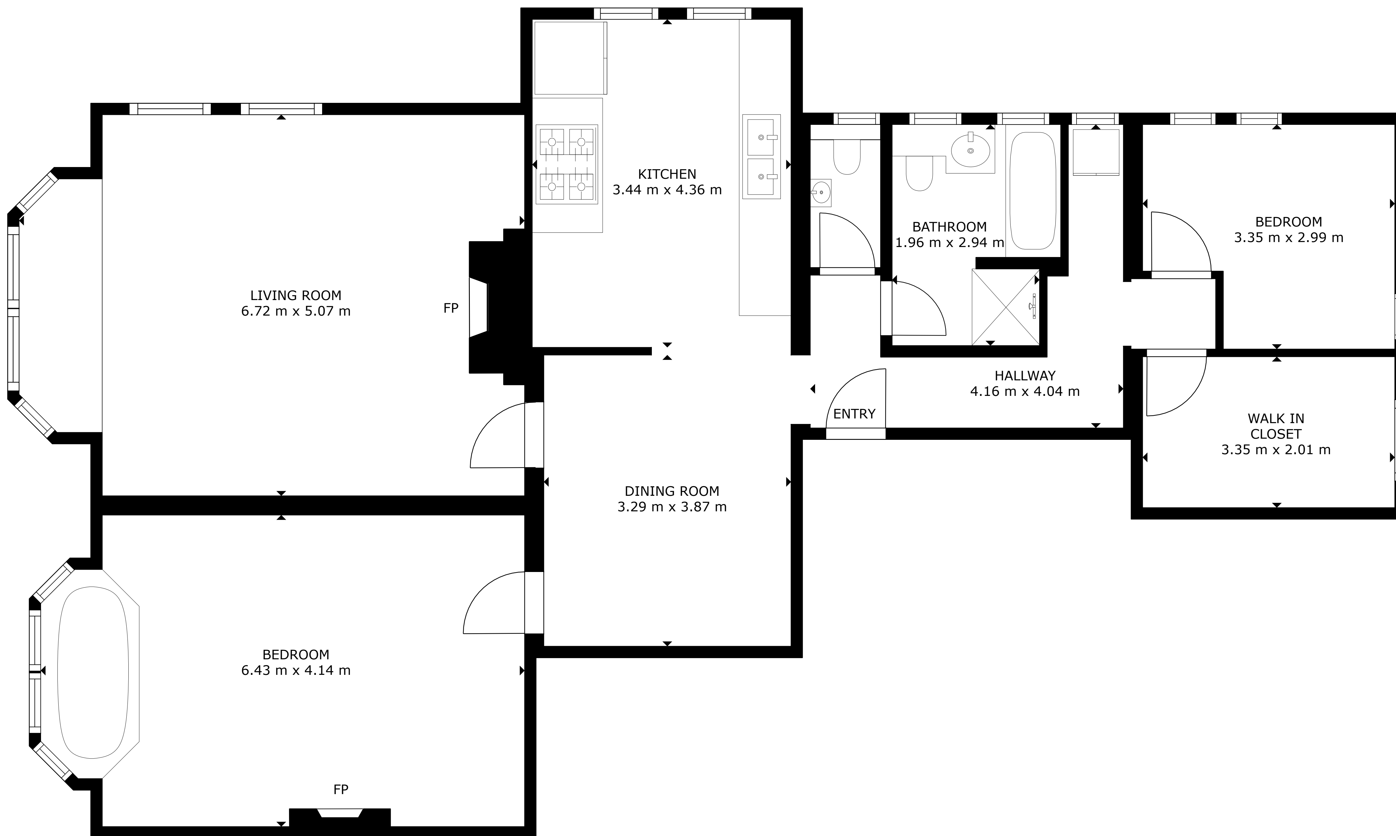
FLOOR PLAN
