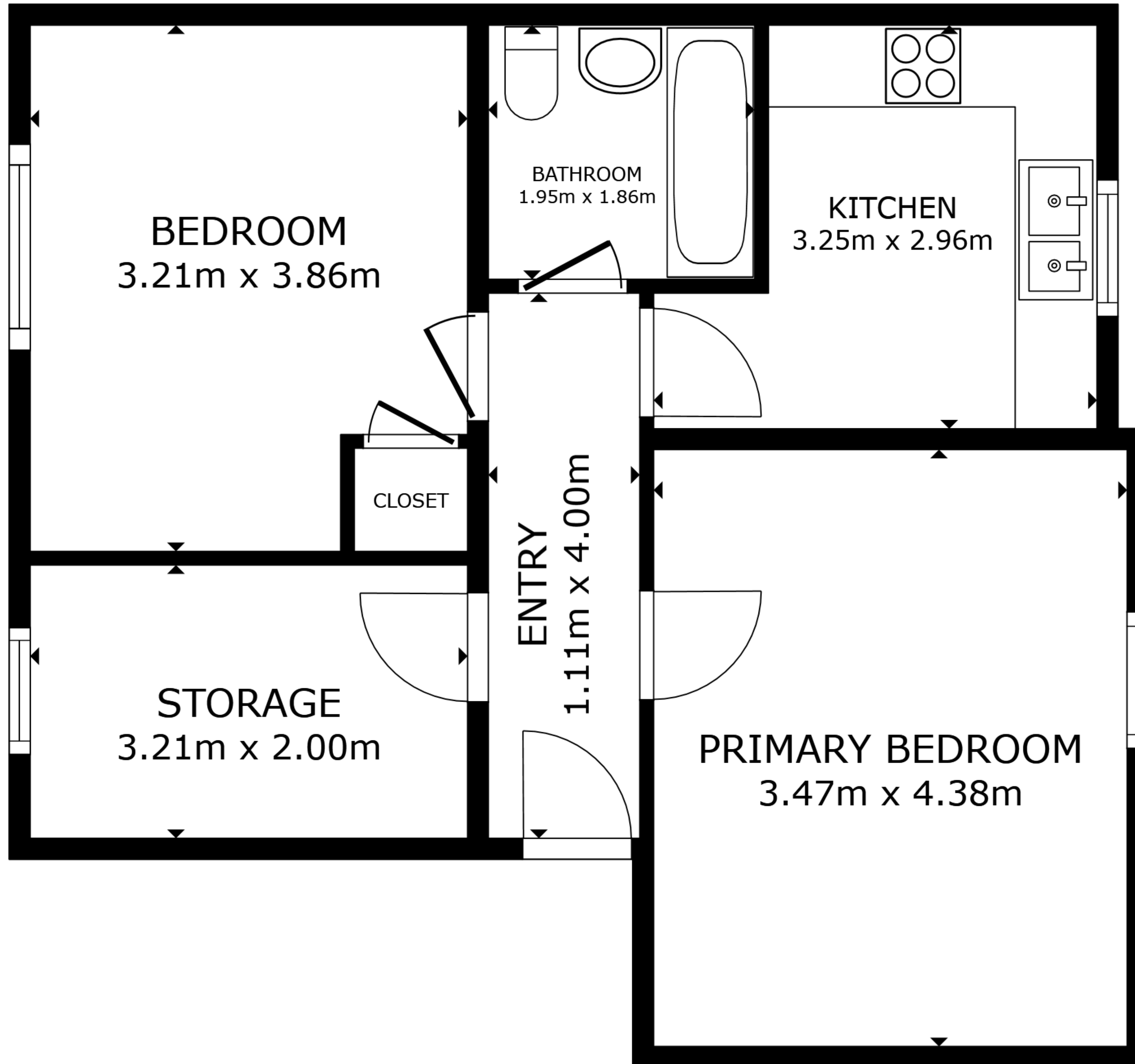
FLOOR PLAN
