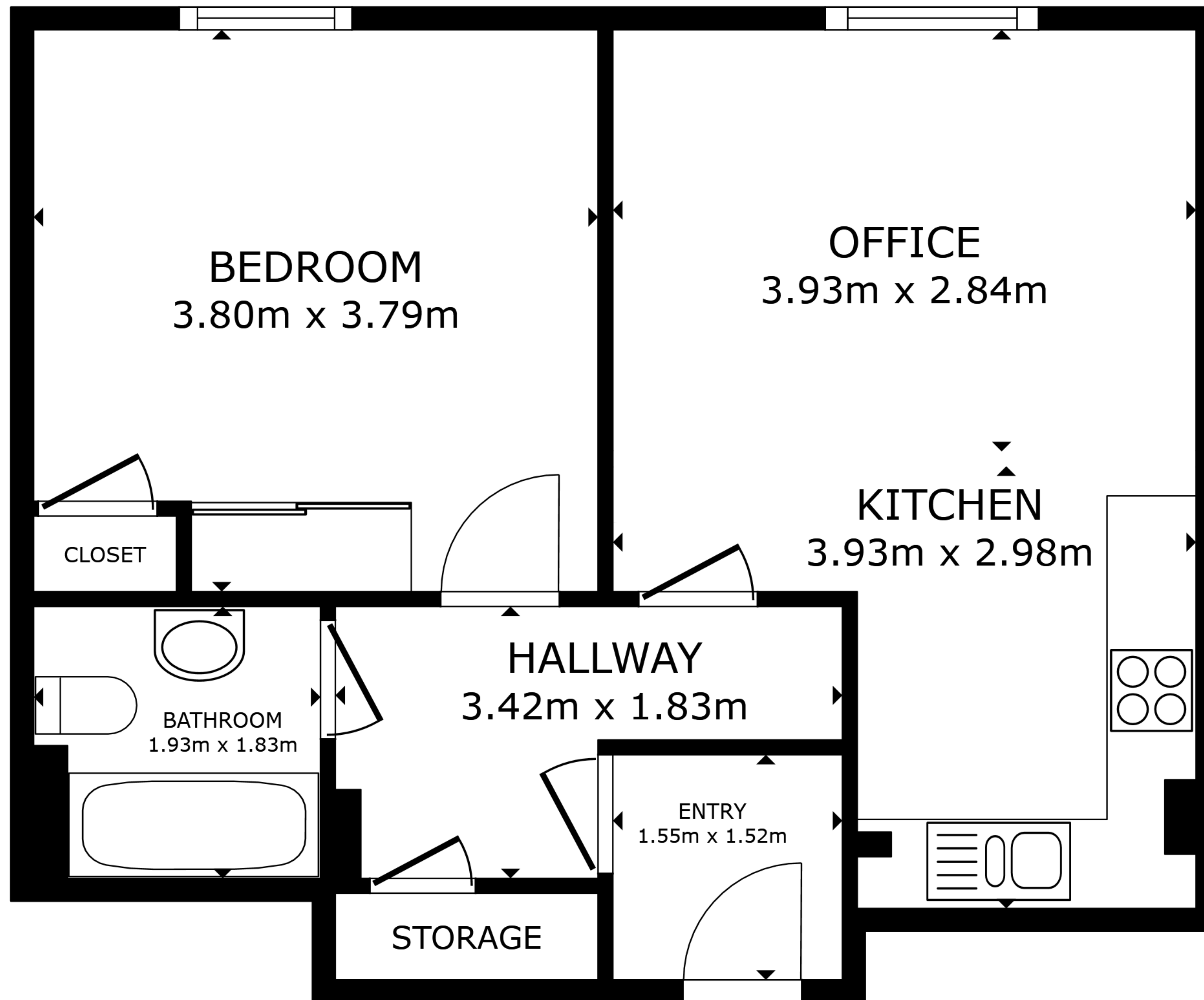
FLOOR PLAN
