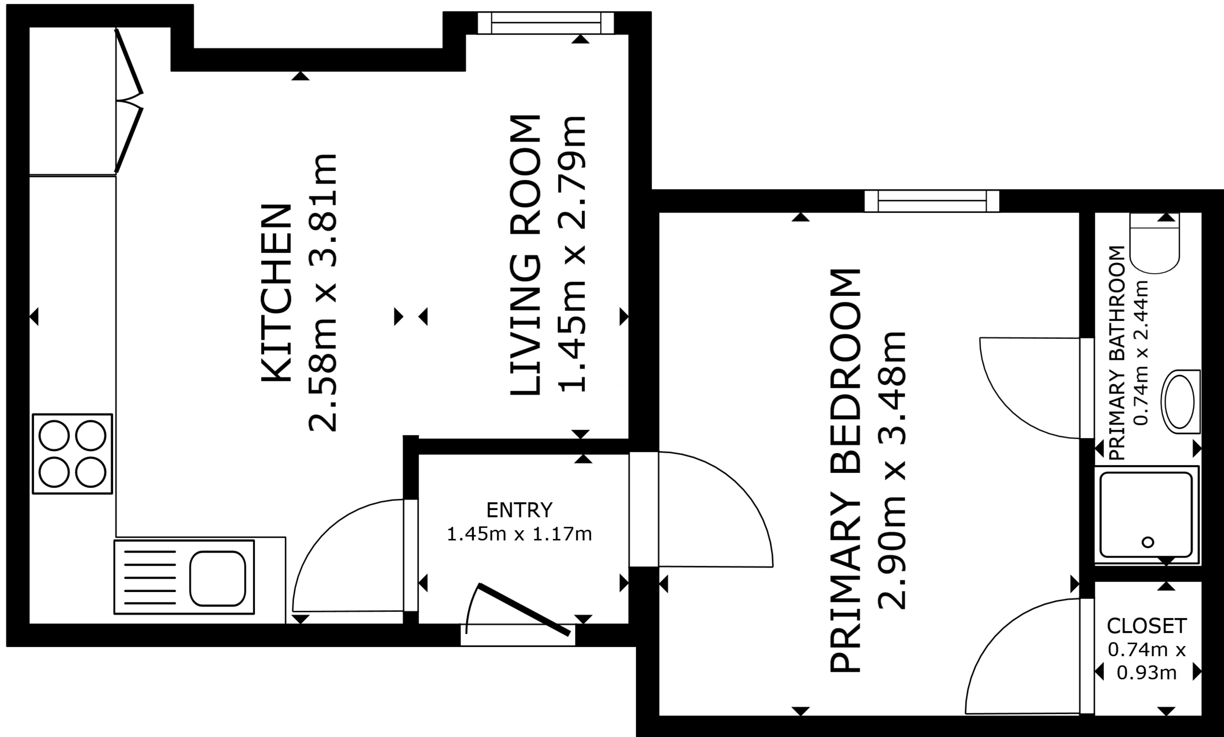
FLOOR PLAN
