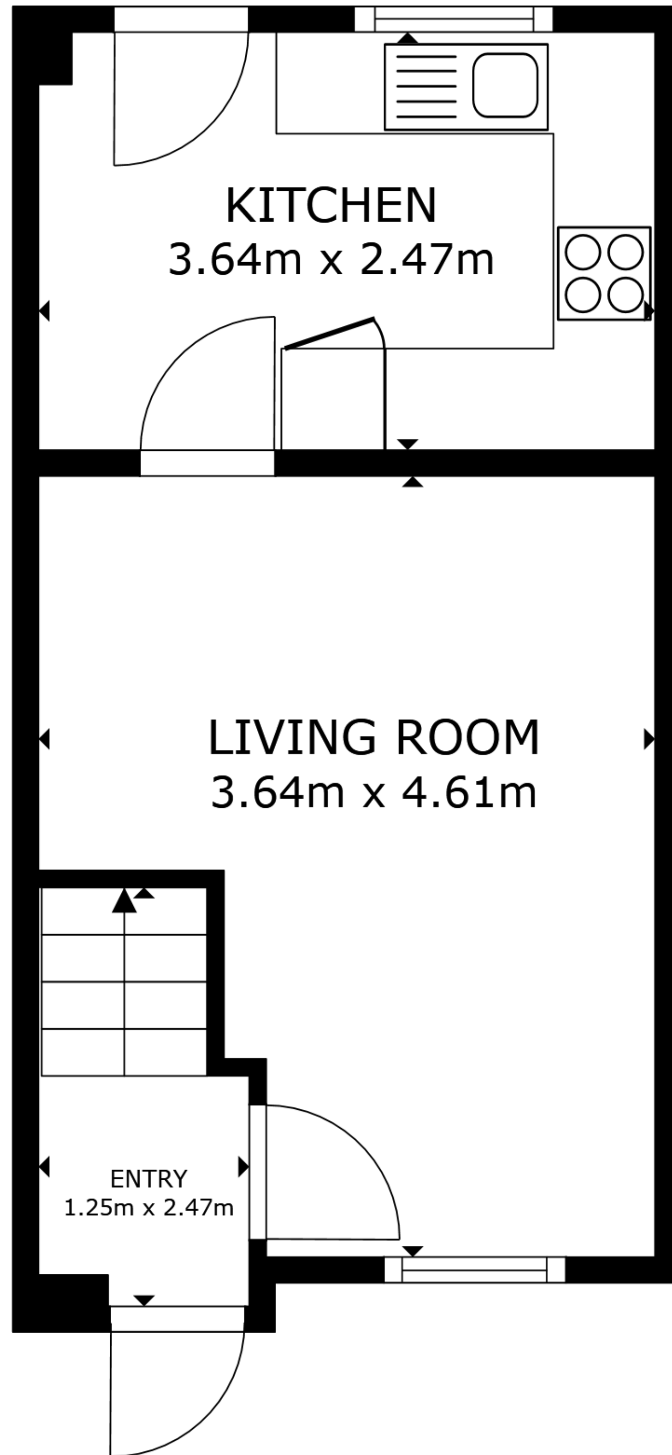
FLOOR 1
