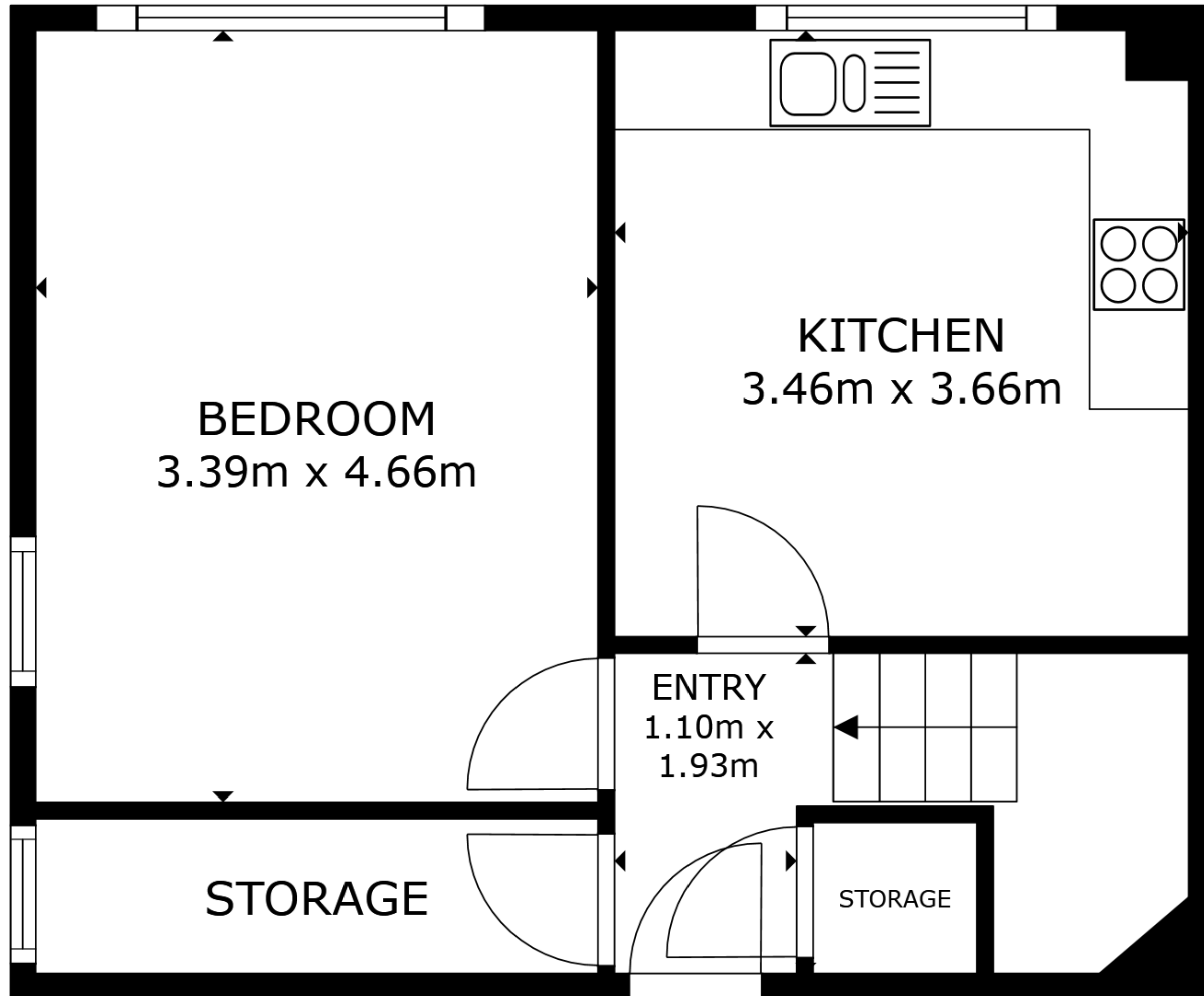
FLOOR 1
