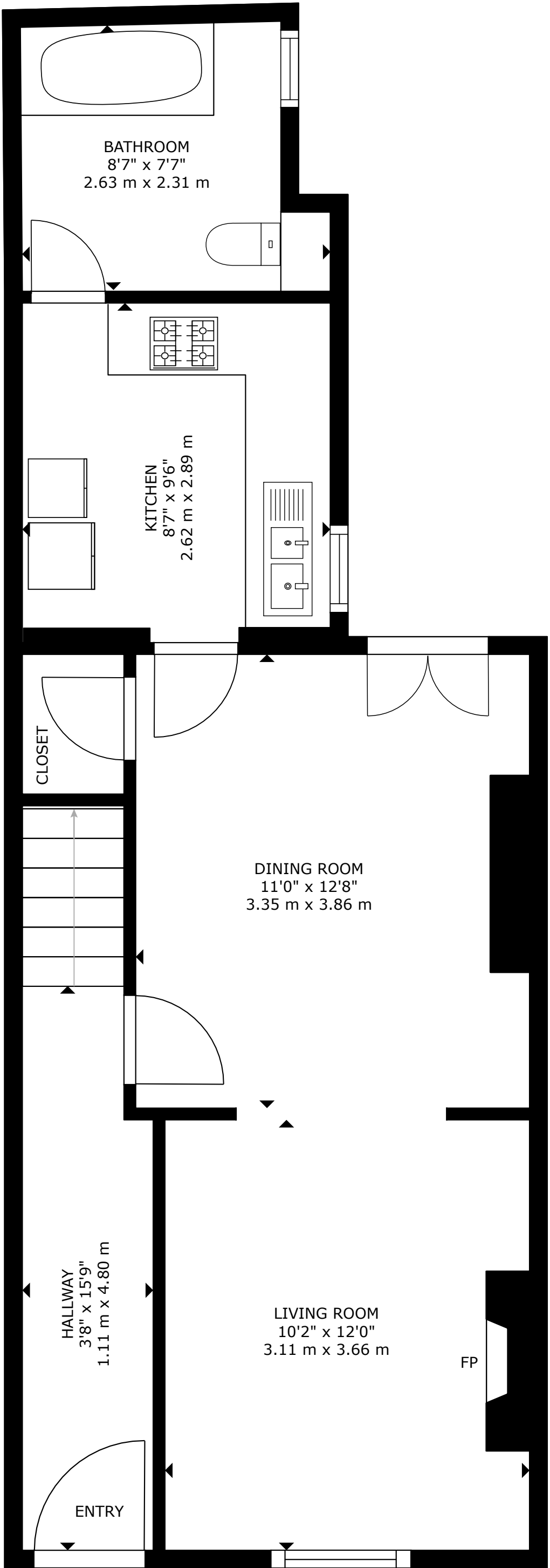
FLOOR 1
