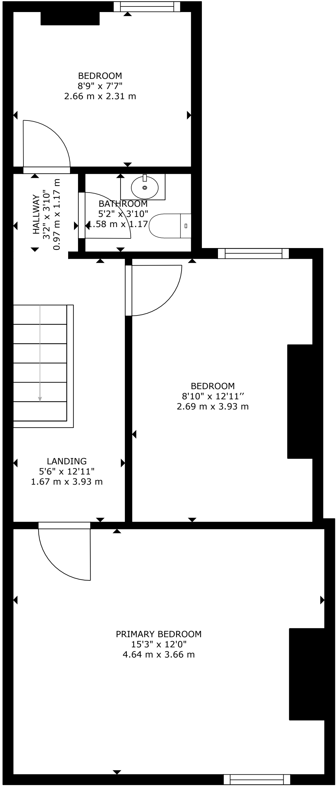
FLOOR 2
