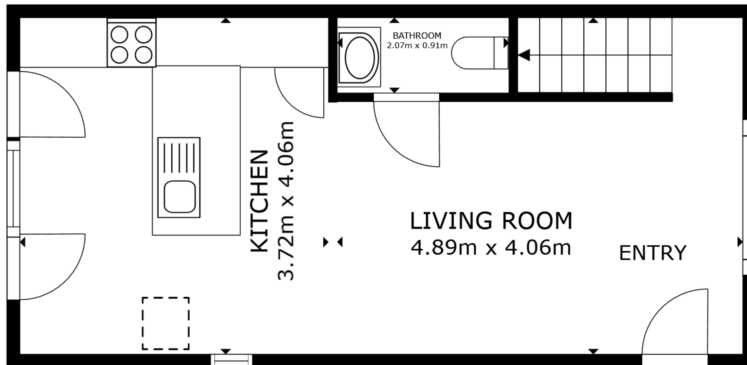
FLOOR 1
