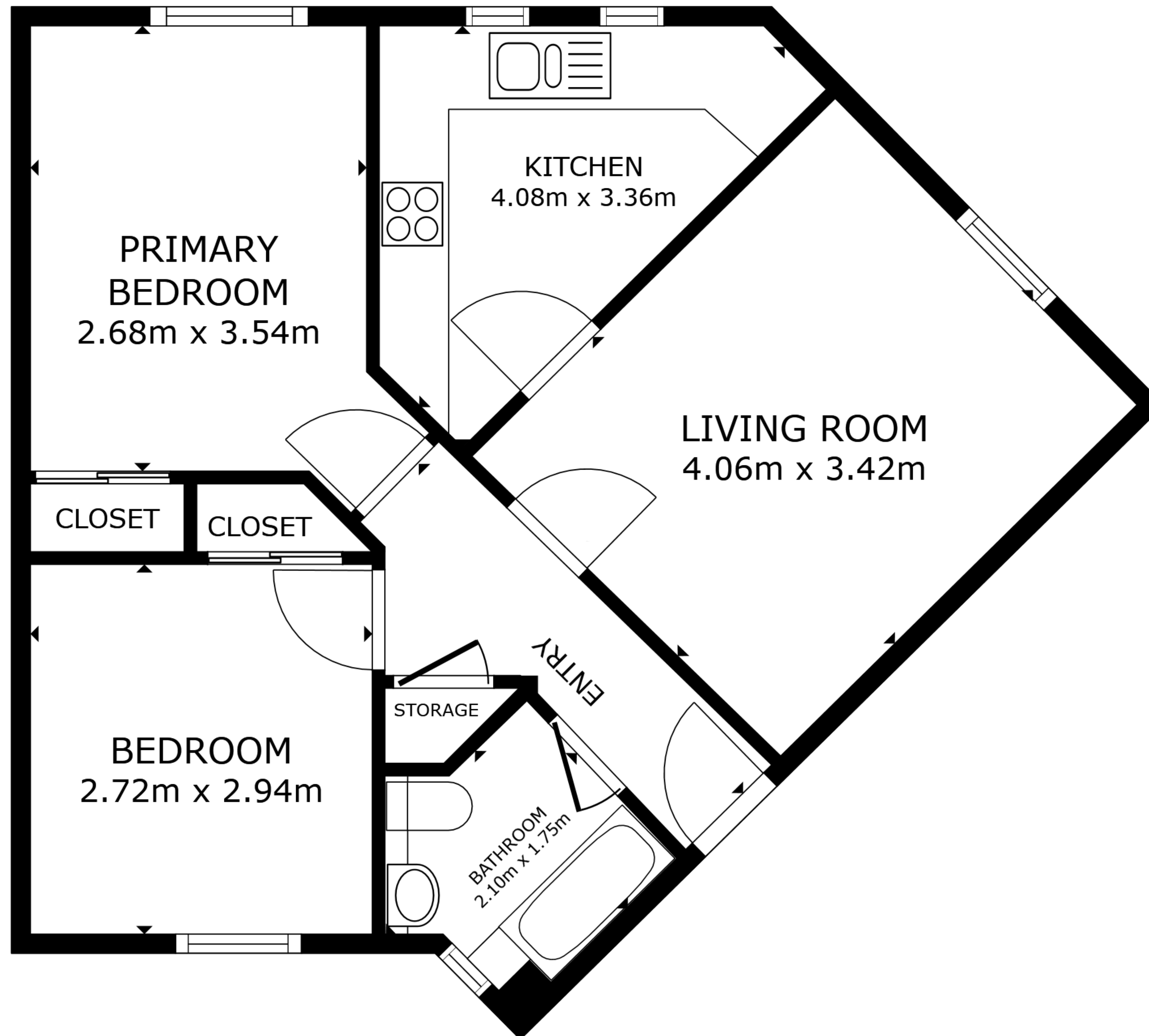
FLOOR PLAN
