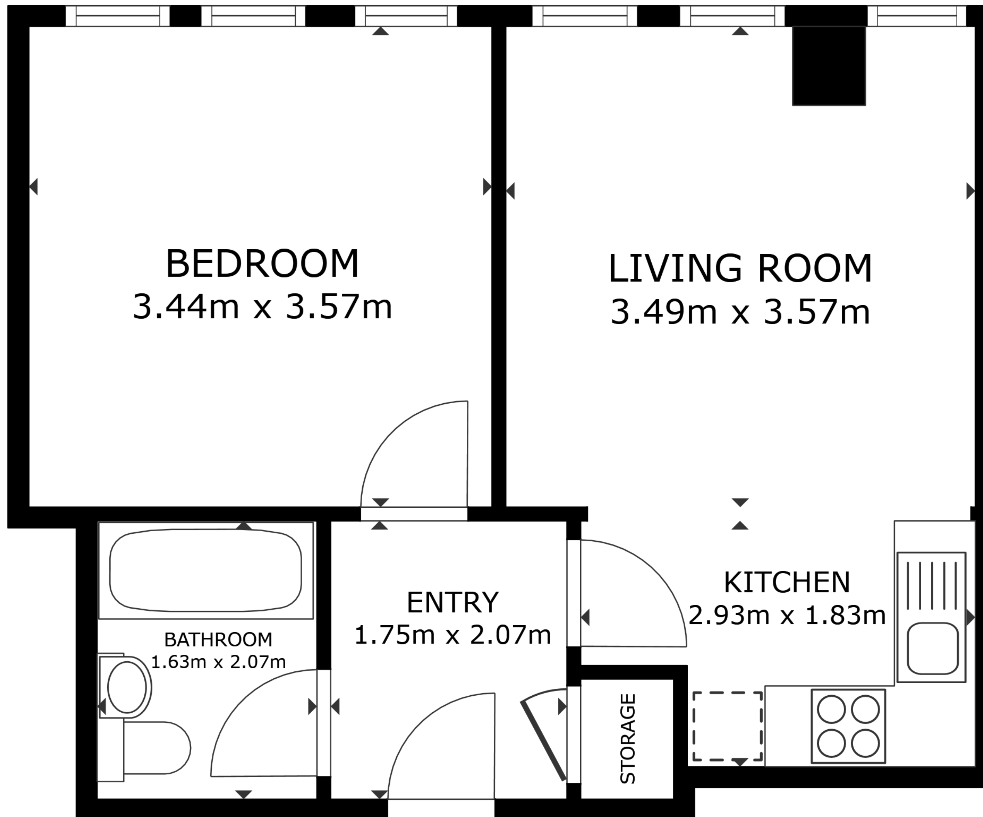
FLOOR PLAN
