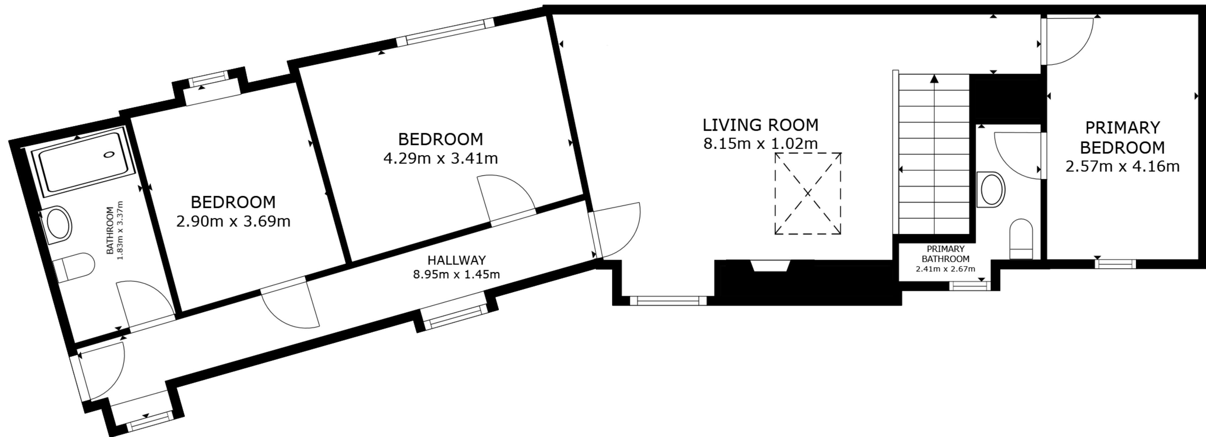
FLOOR 2
