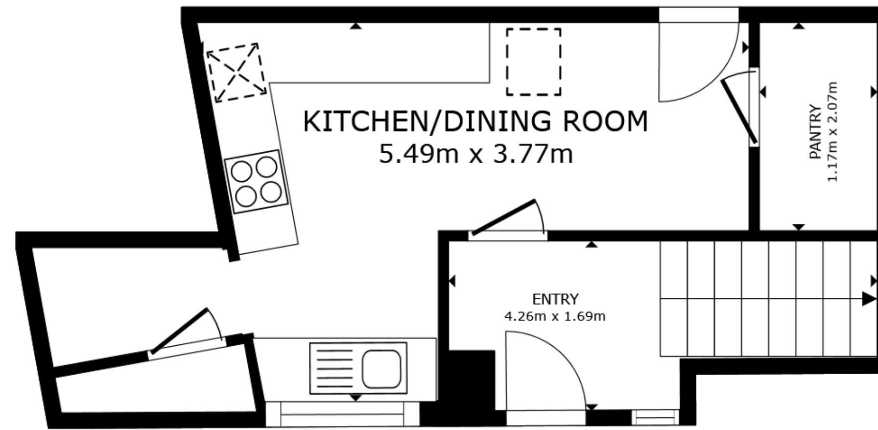
FLOOR 1
