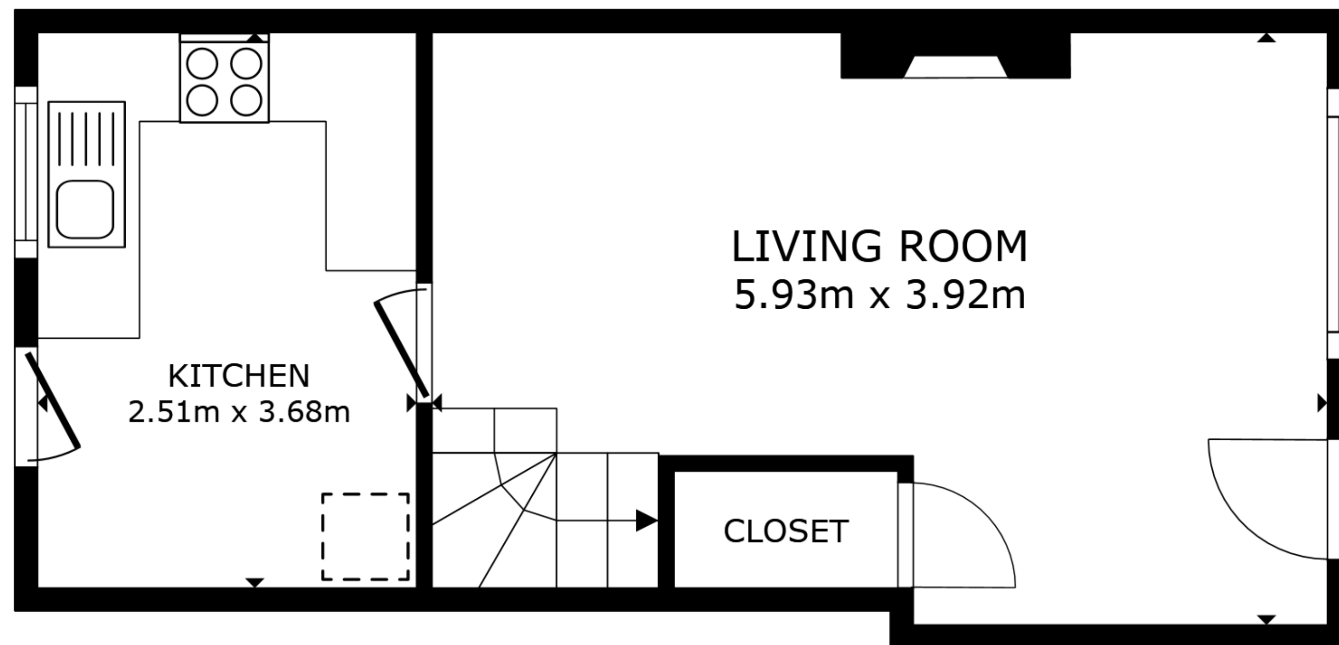
FLOOR 1
