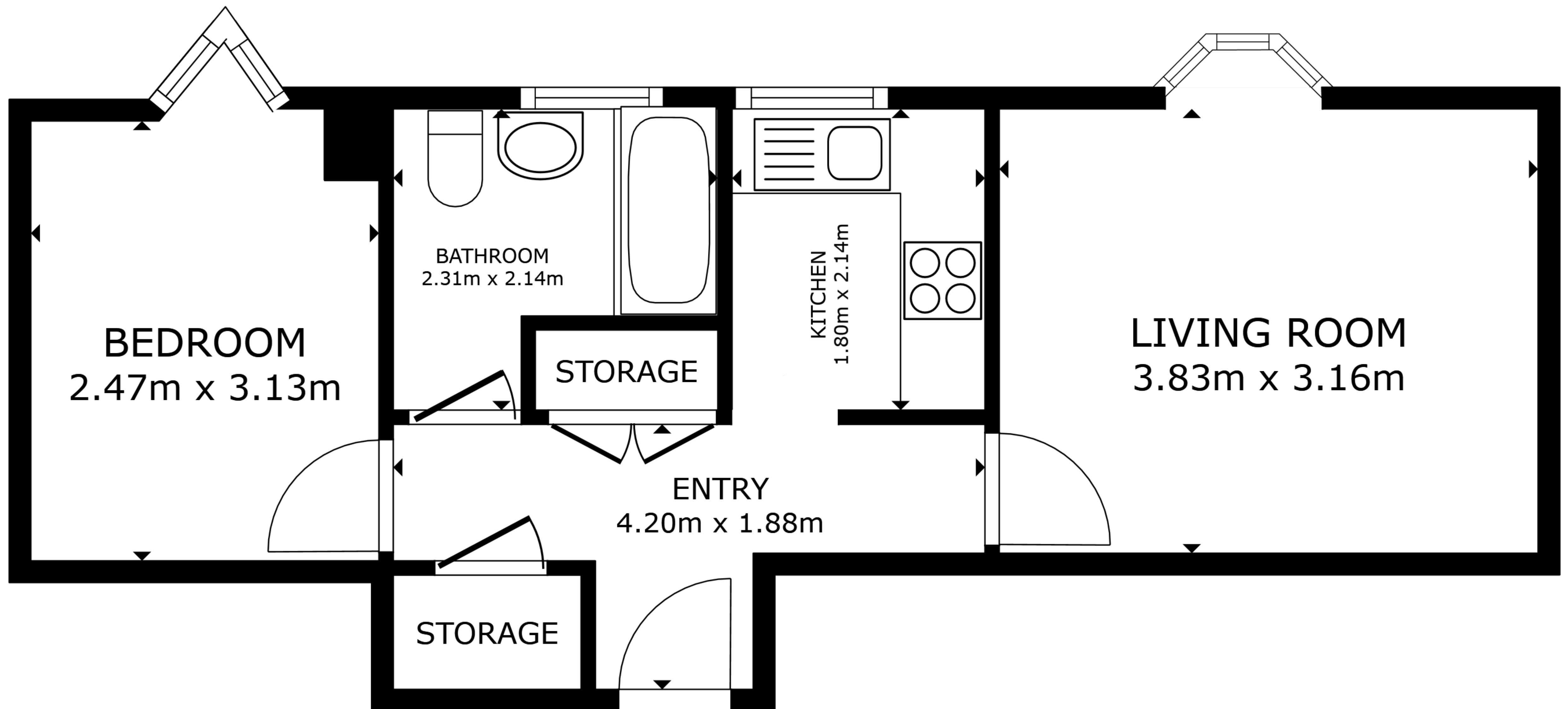
FLOOR PLAN
