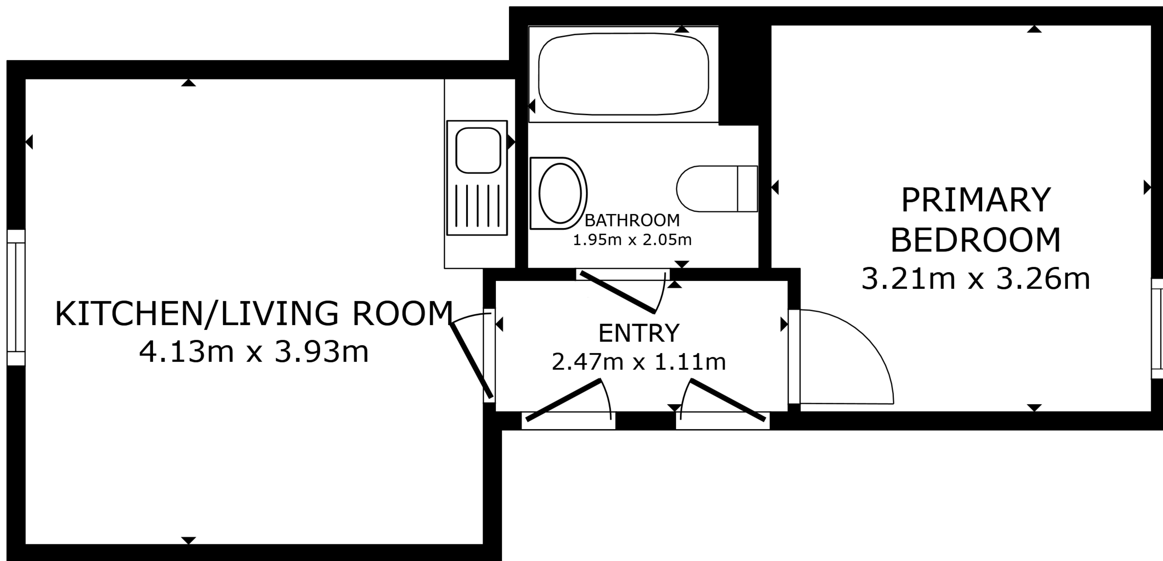
FLOOR PLAN
