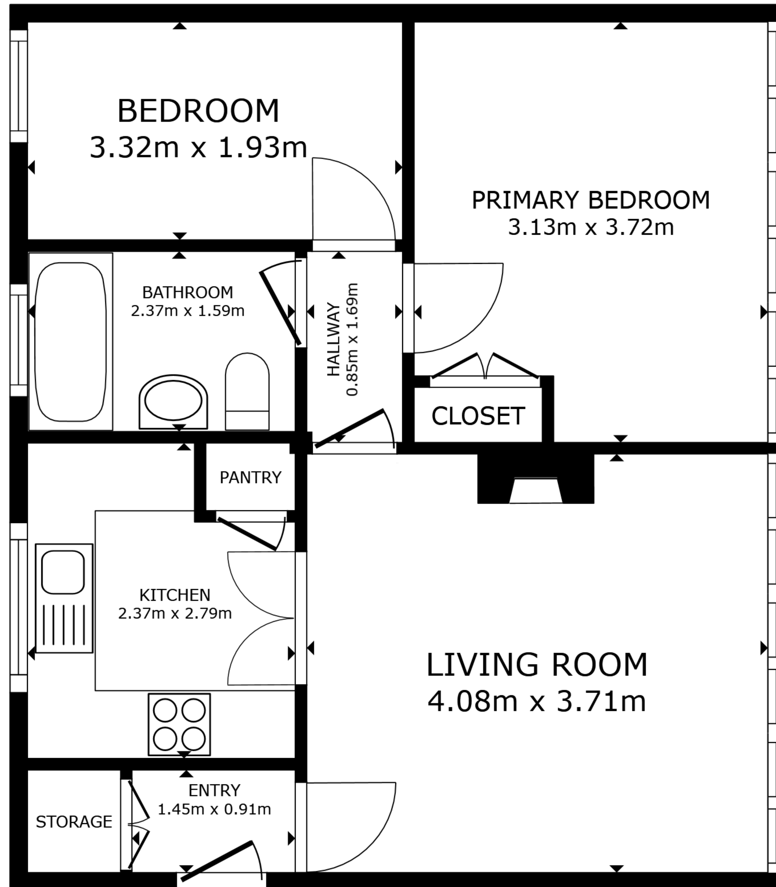
FLOOR PLAN
