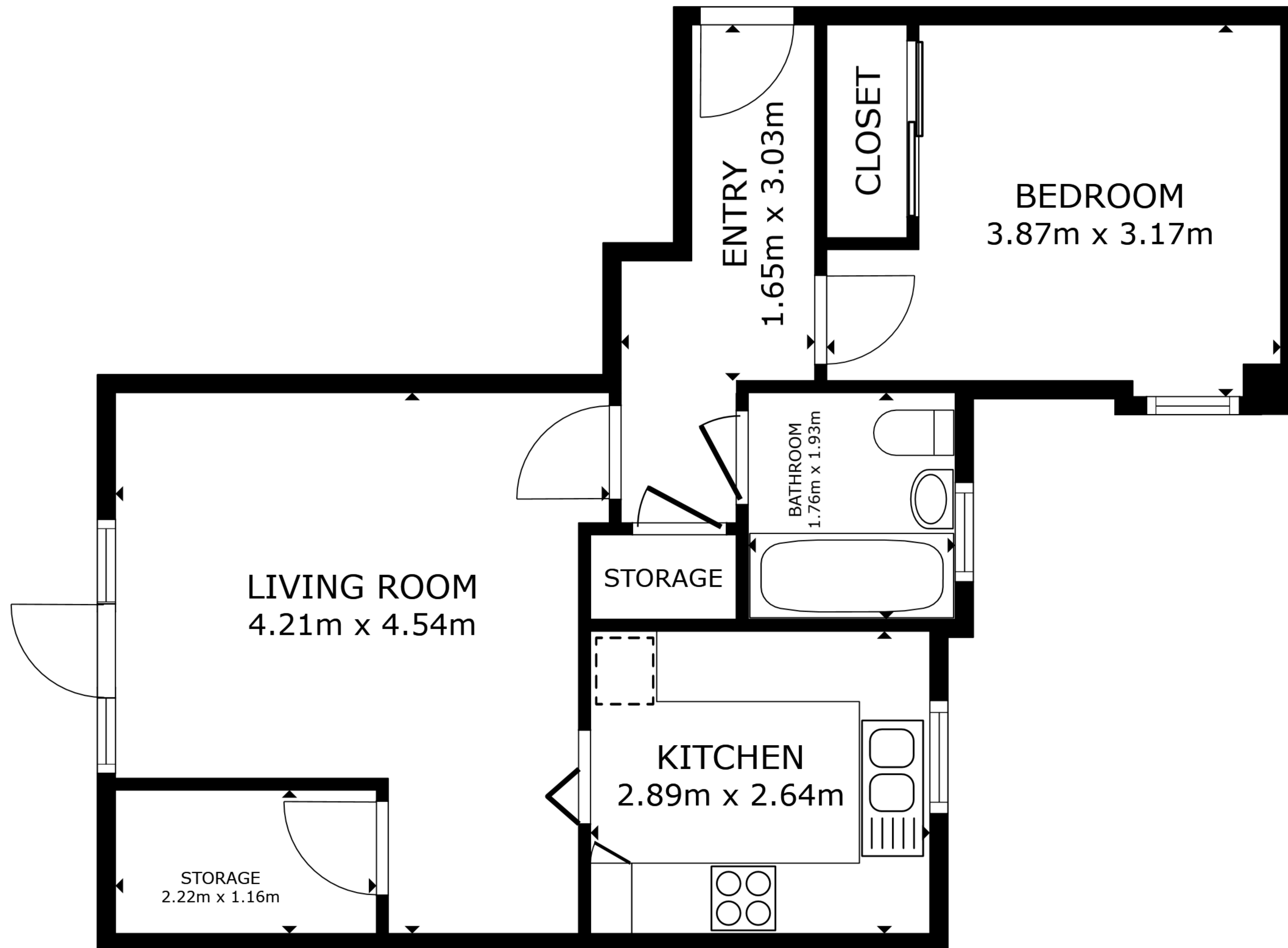
FLOOR PLAN
