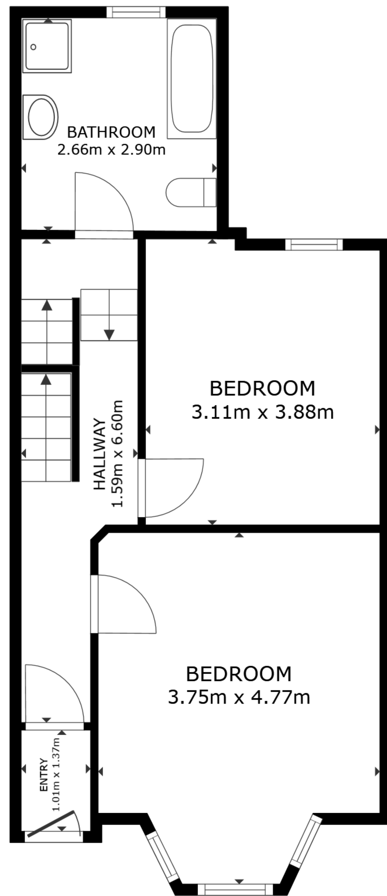
FLOOR 1
