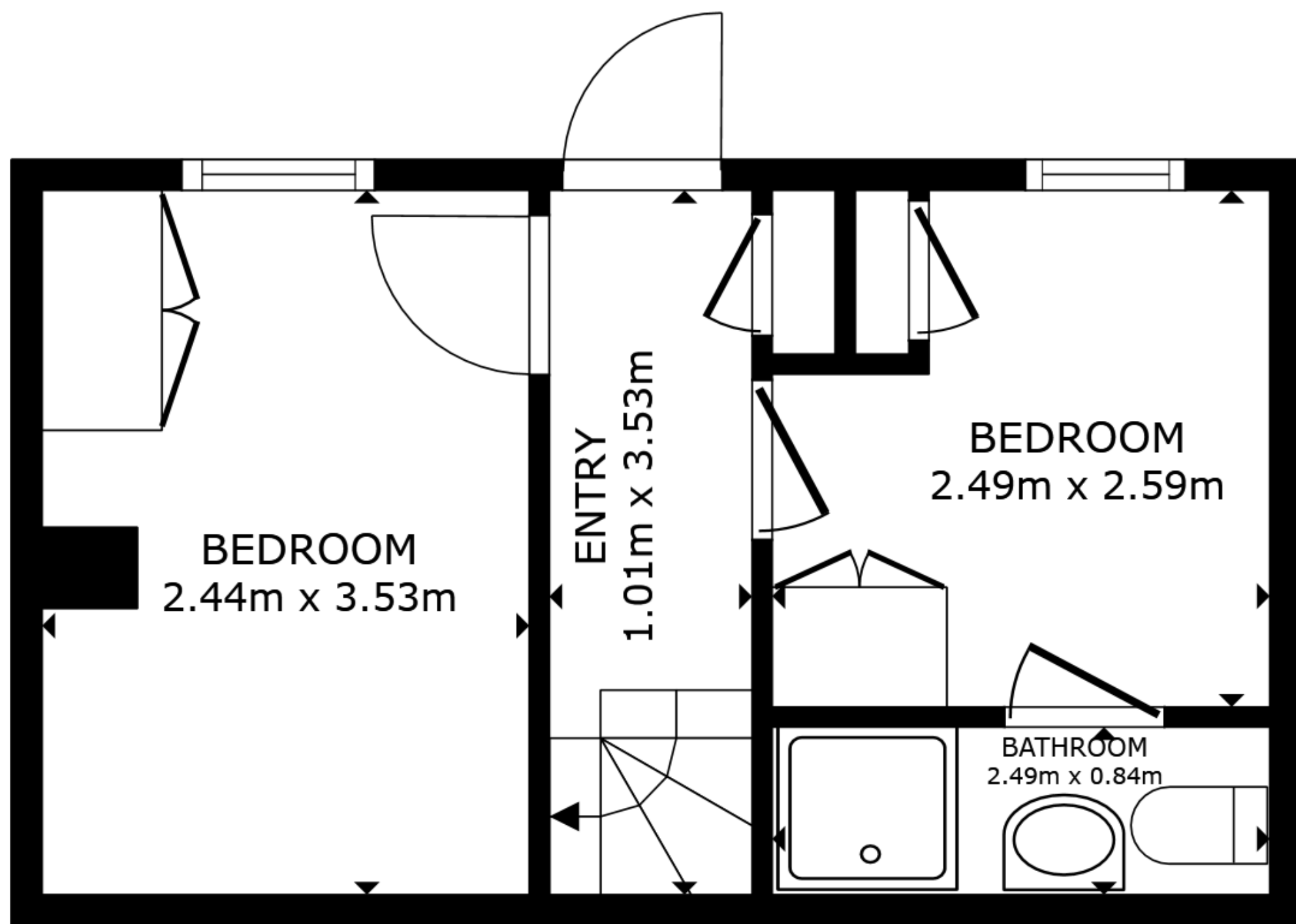
FLOOR 1
