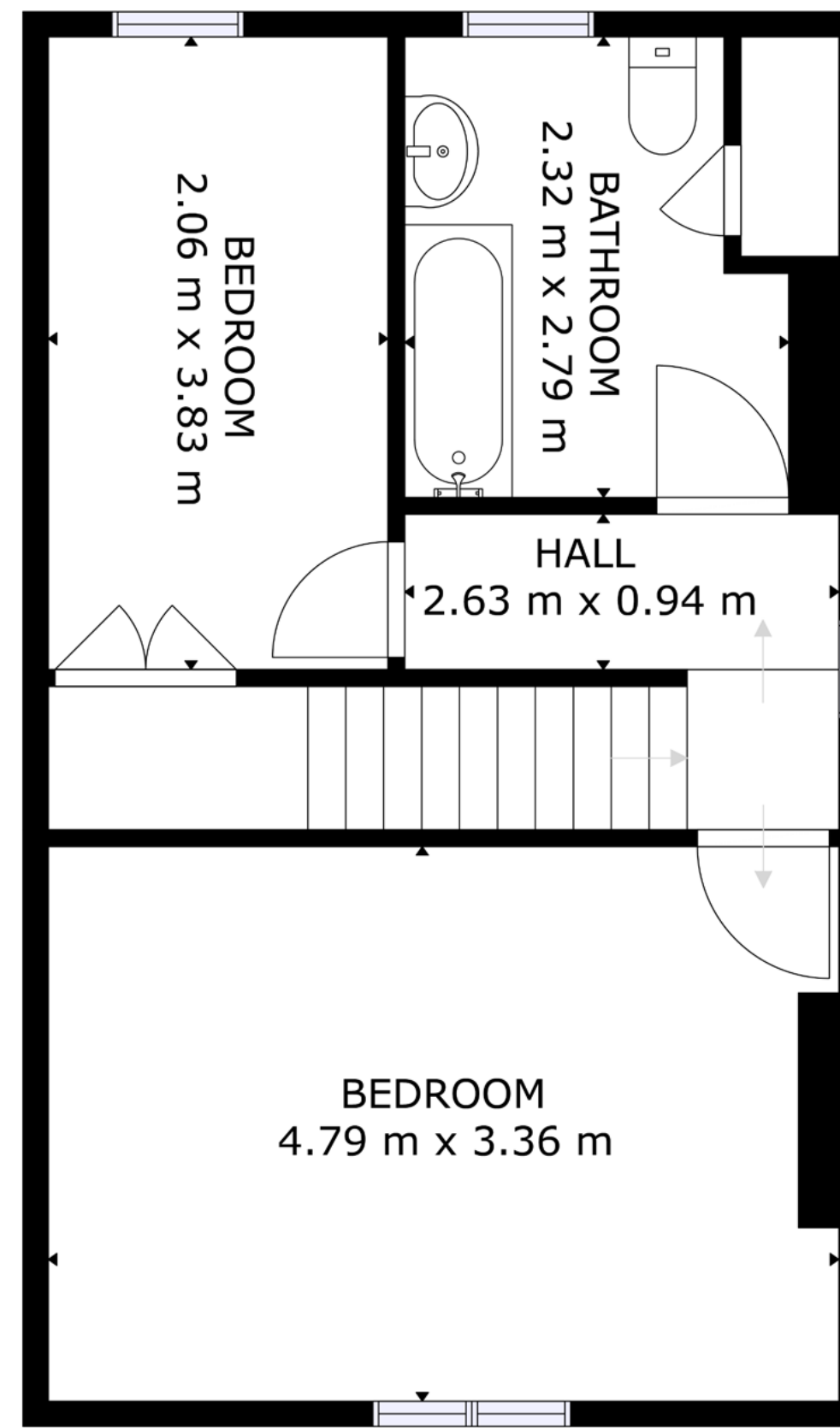
FLOOR 2
