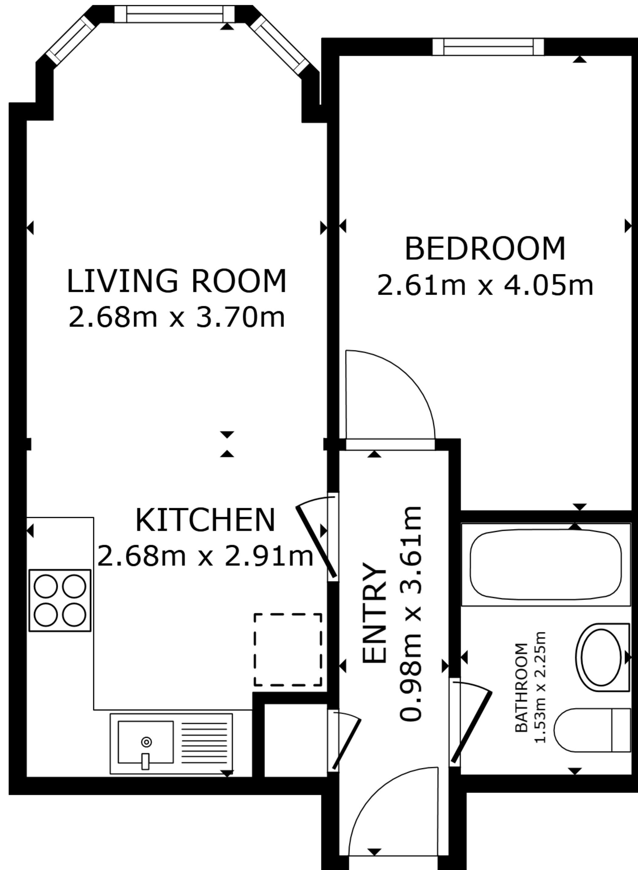
FLOOR PLAN
