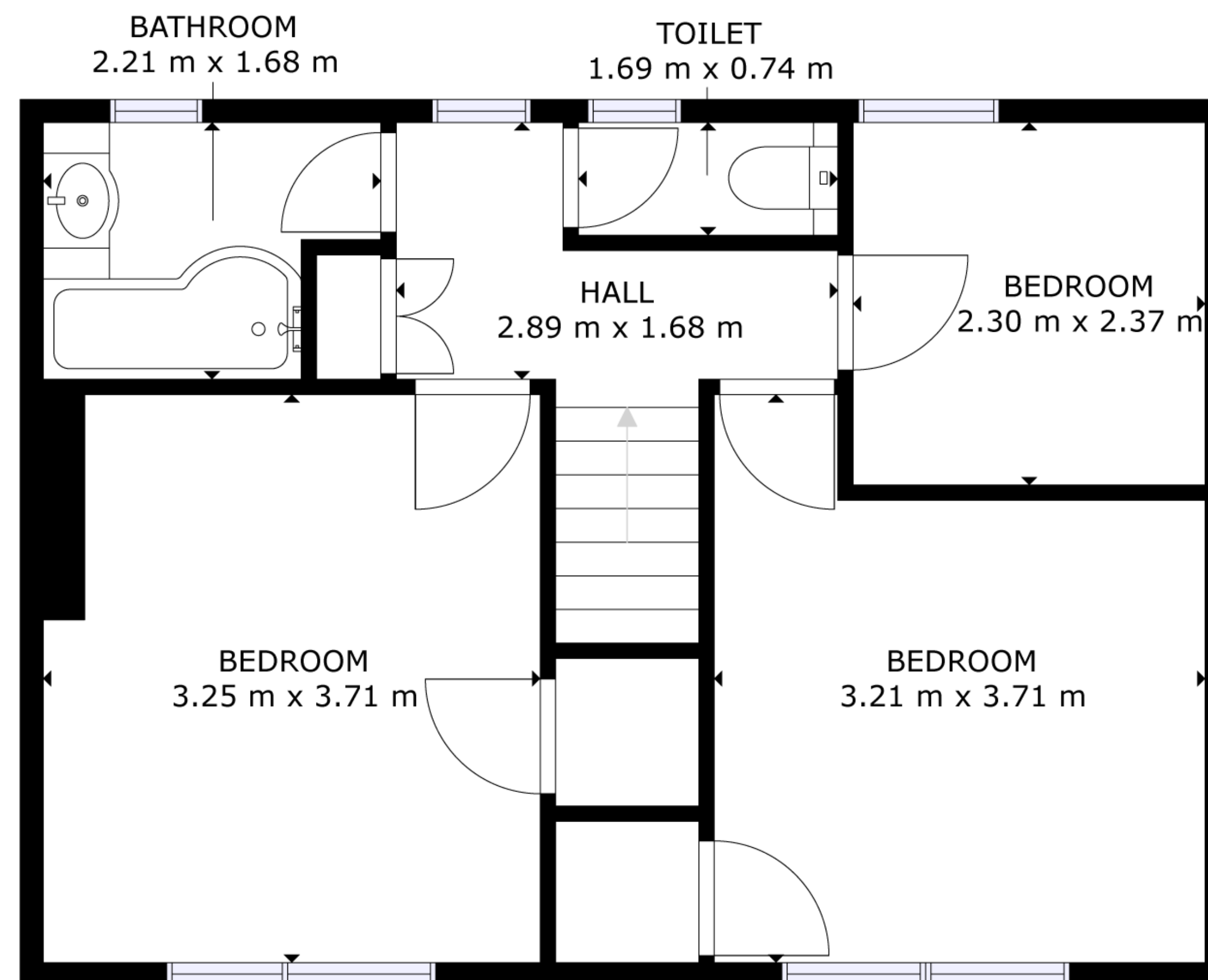
FLOOR 2
