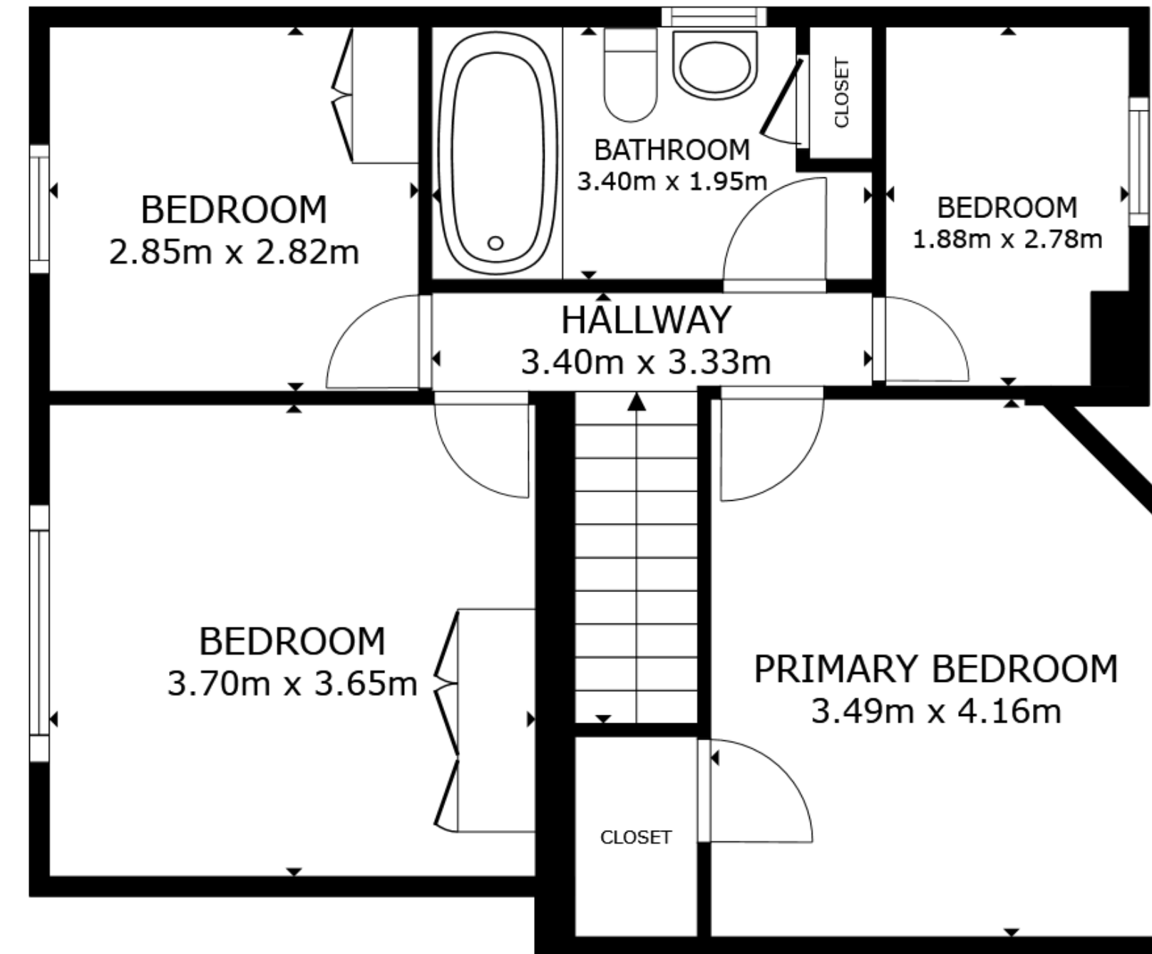
FLOOR 2
