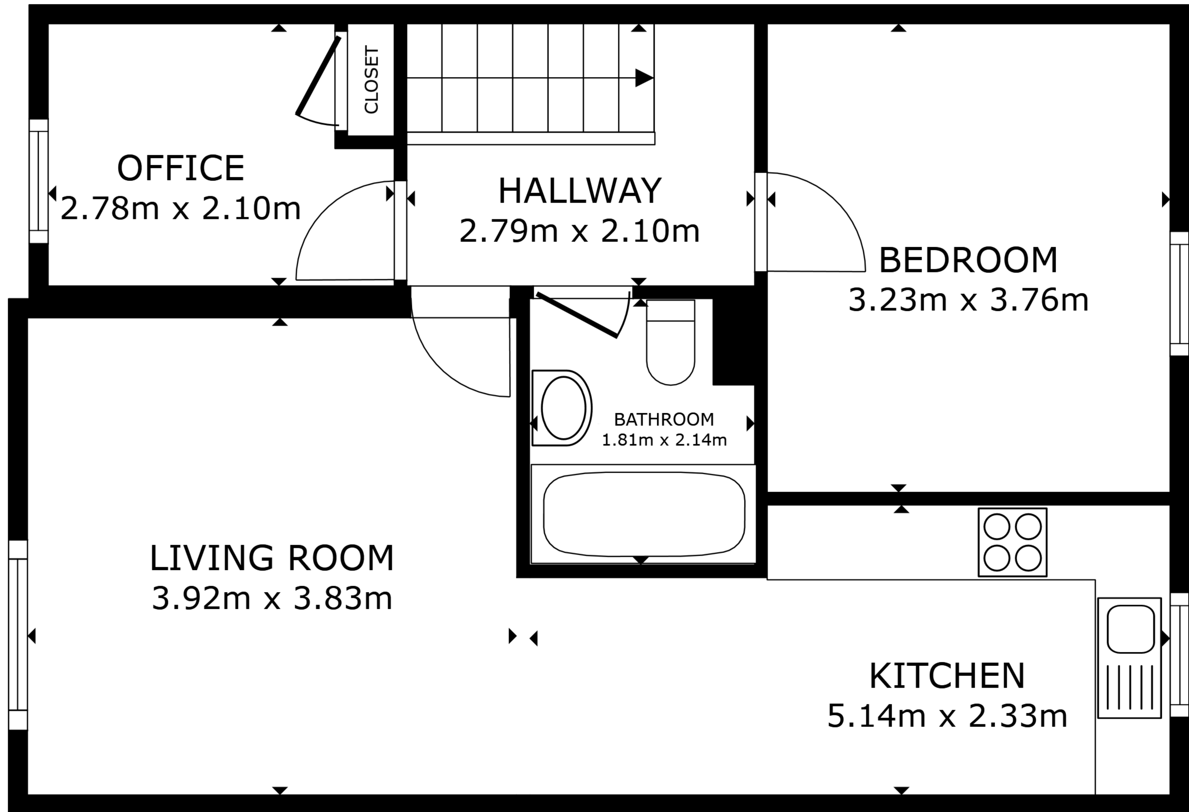
FLOOR PLAN
